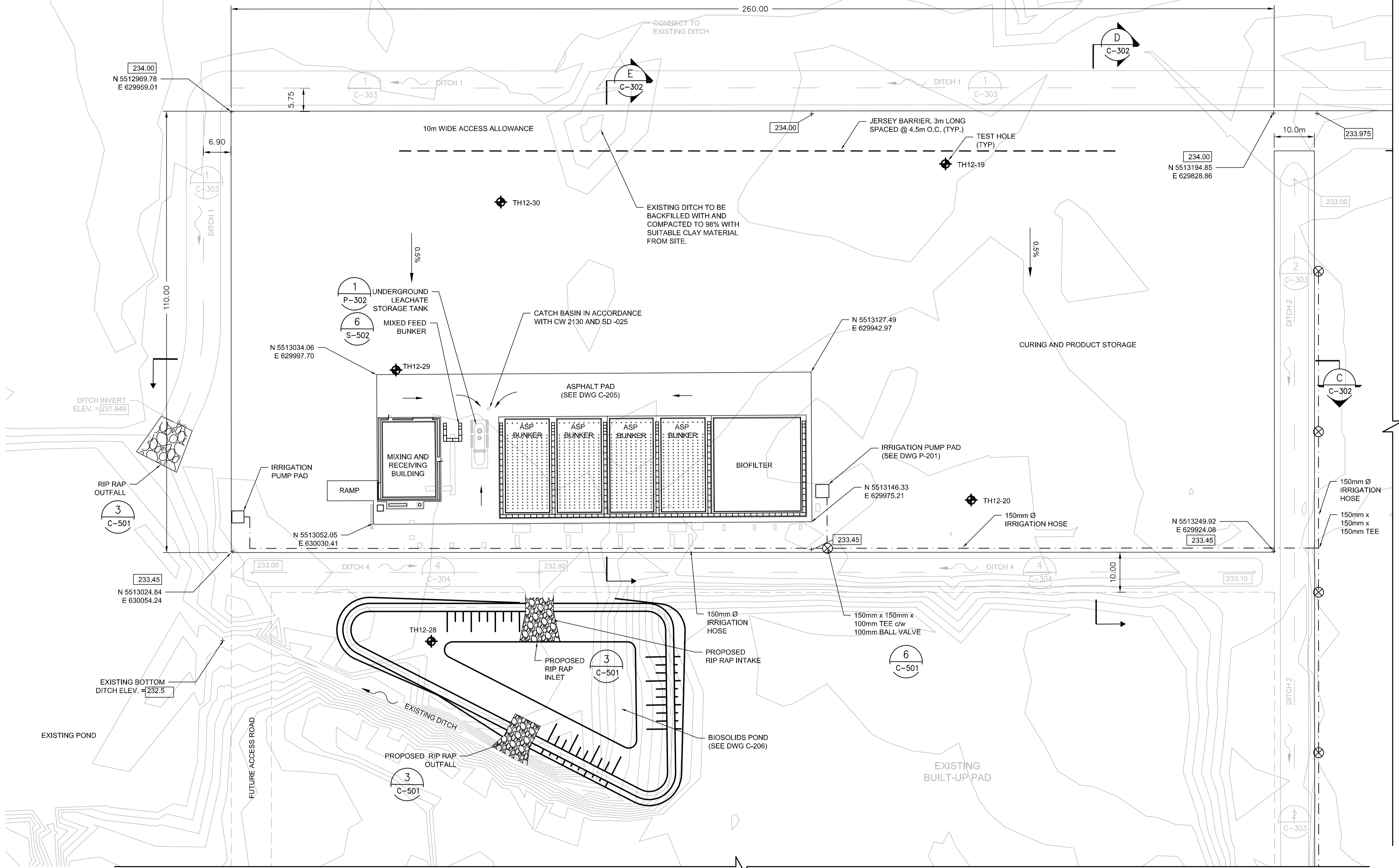
1 PLAN 1:500
