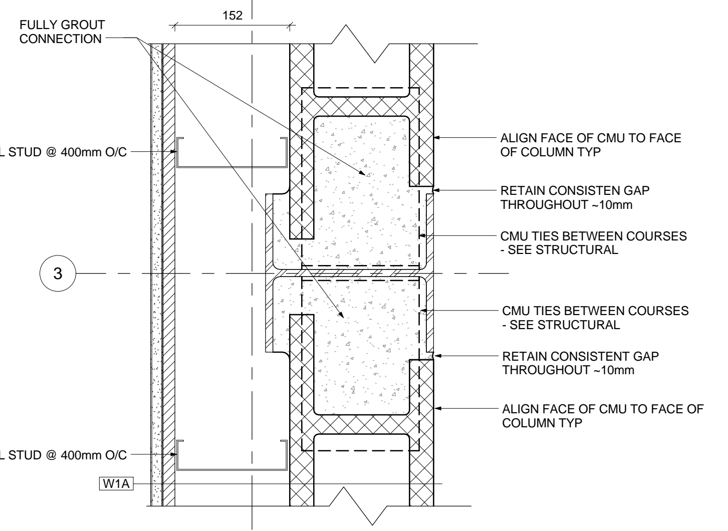
5 TYP PLAN DETAIL @ BLOCK INFILL / FURRING WALL 1:5
