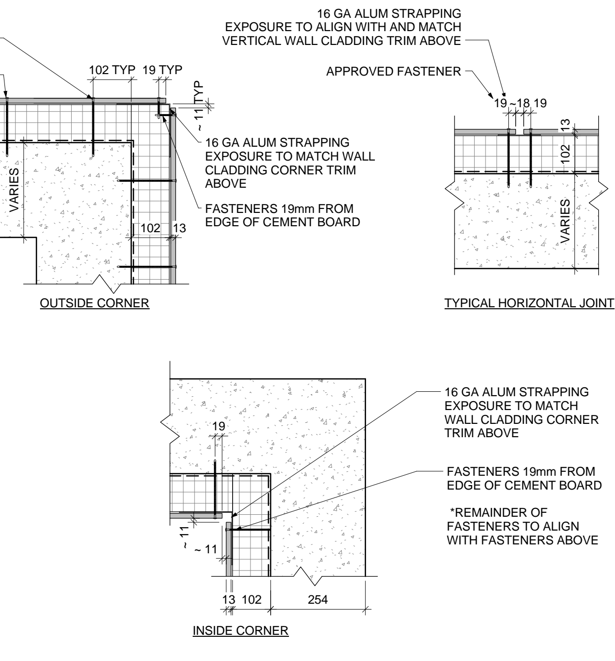
12 FOUNDATION CLADDING DETAILS 1:10
