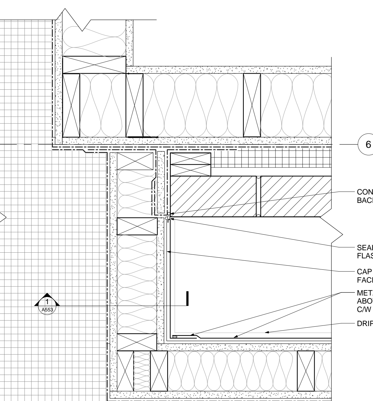
9 PLAN DETAIL - WEST VESTIBULE PARAPET ABOVE 1:5
