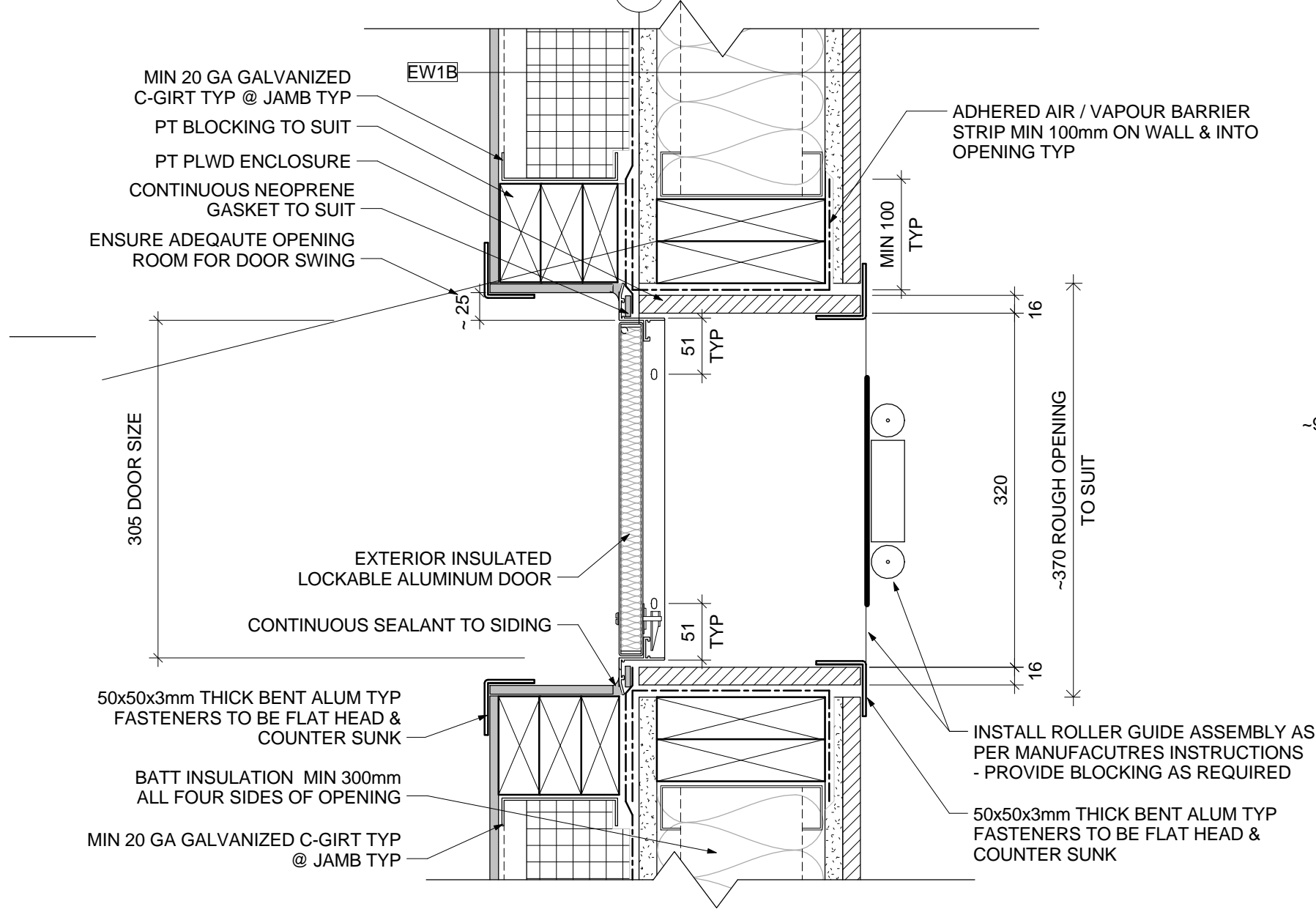
4 PLAN DETAIL - HOSE ACCESS DOOR 1:5
