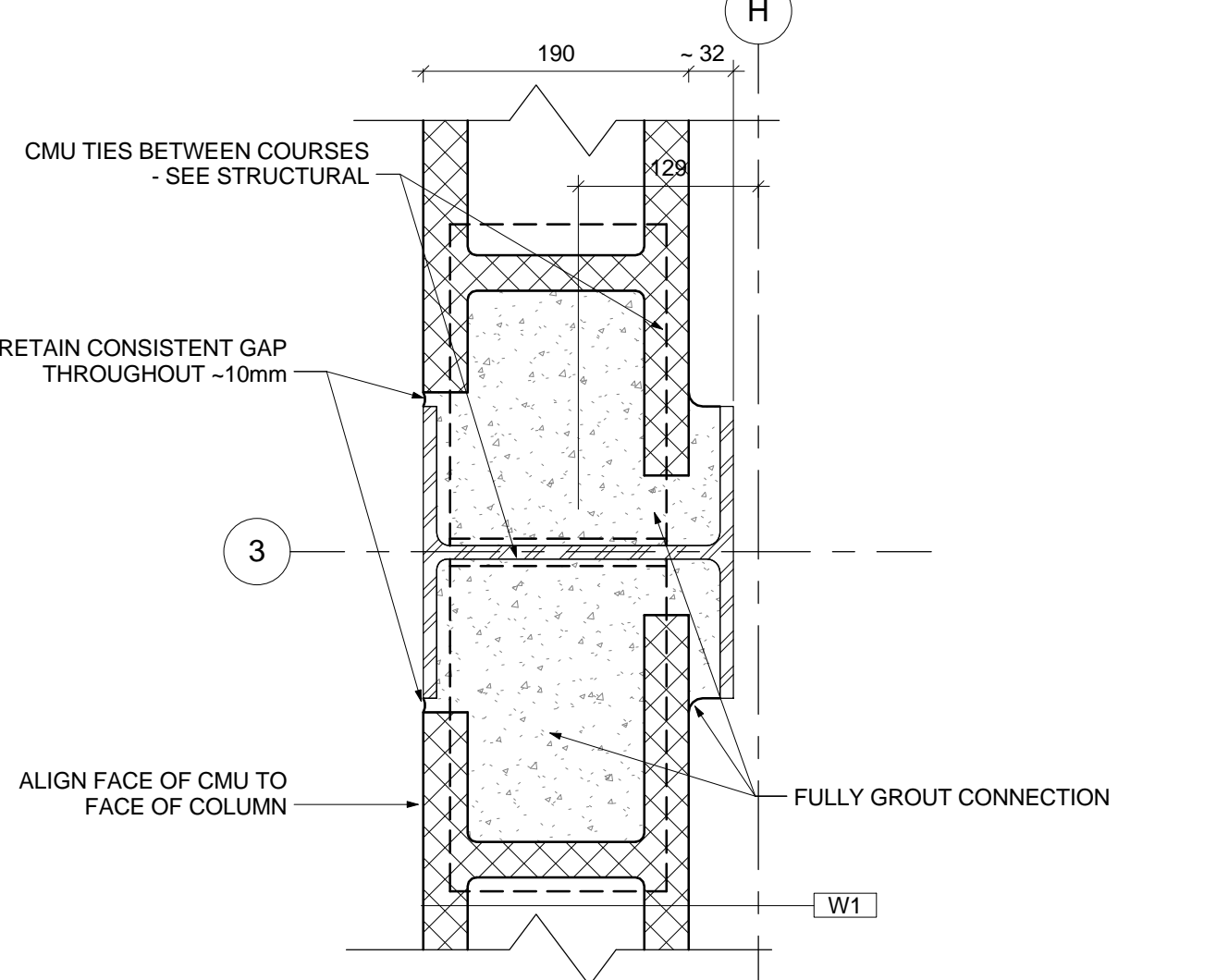
6 TYP PLAN DETAIL - COLUMN @ BLOCK INFILL 1:5
