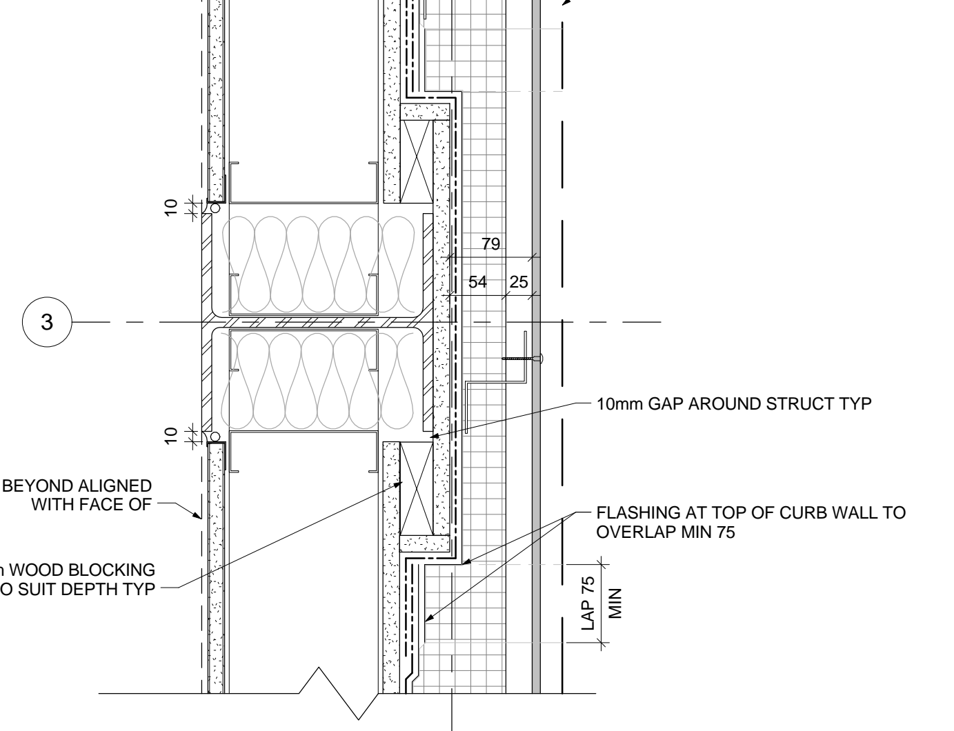
13 TYP PLAN DETAIL - UPPER GYM WALL @ COLUMN 1:5
