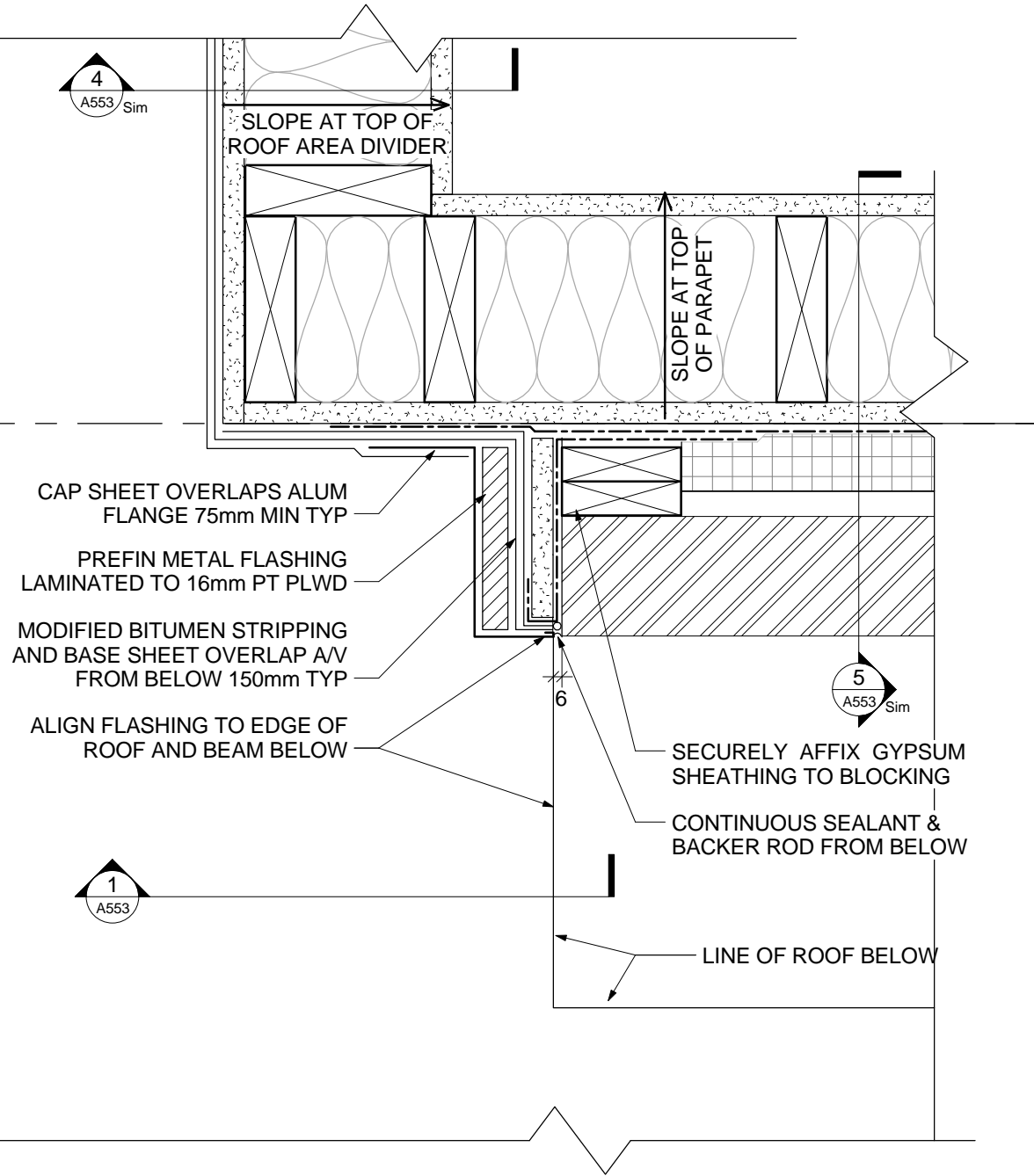
8 PLAN DETAIL - WEST VESTIBULE PARAPET 1:5
