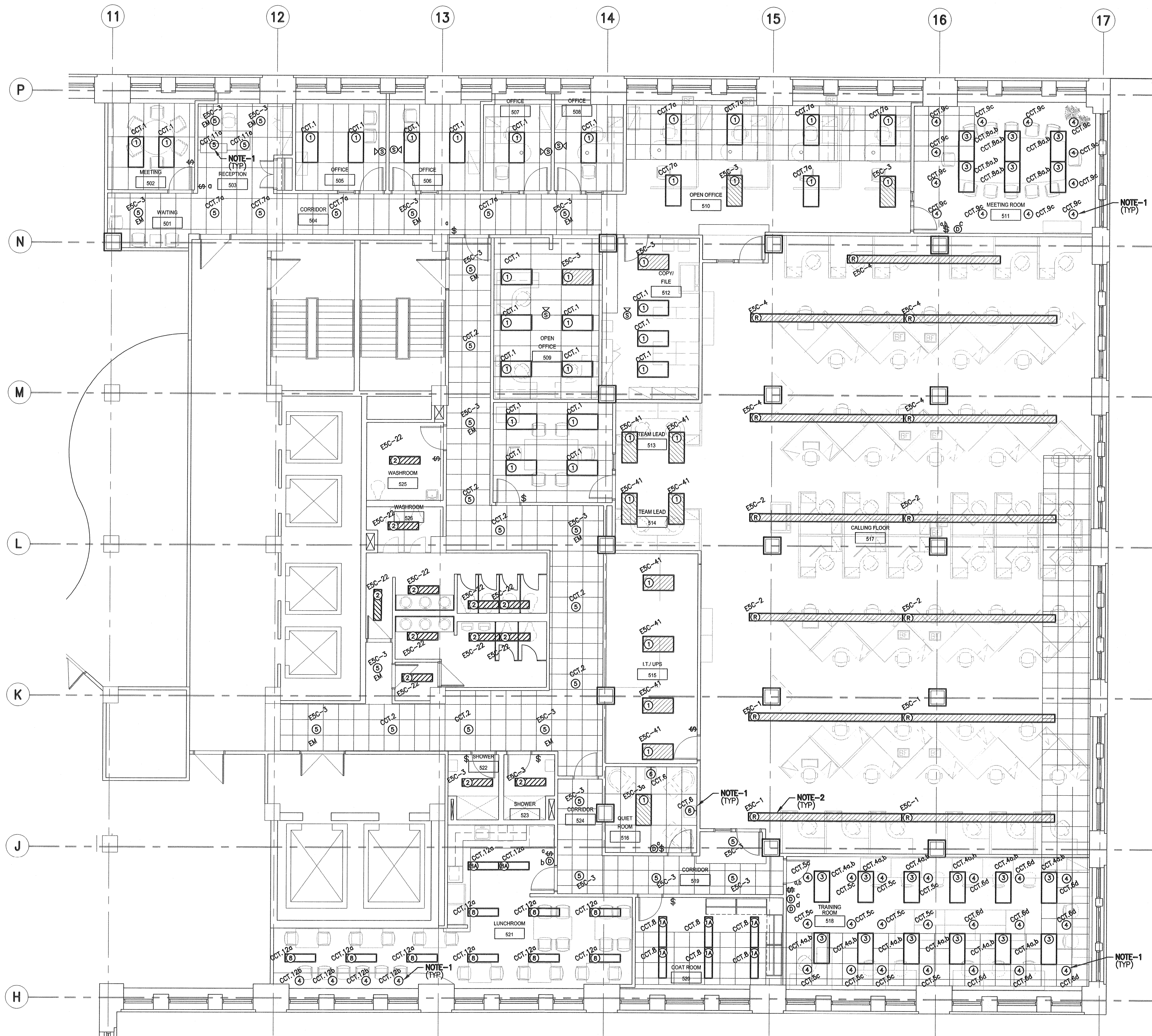
1 FLOOR PLAN - LIGHTING E2.1 SCALE: 1/8"=1'-0"
