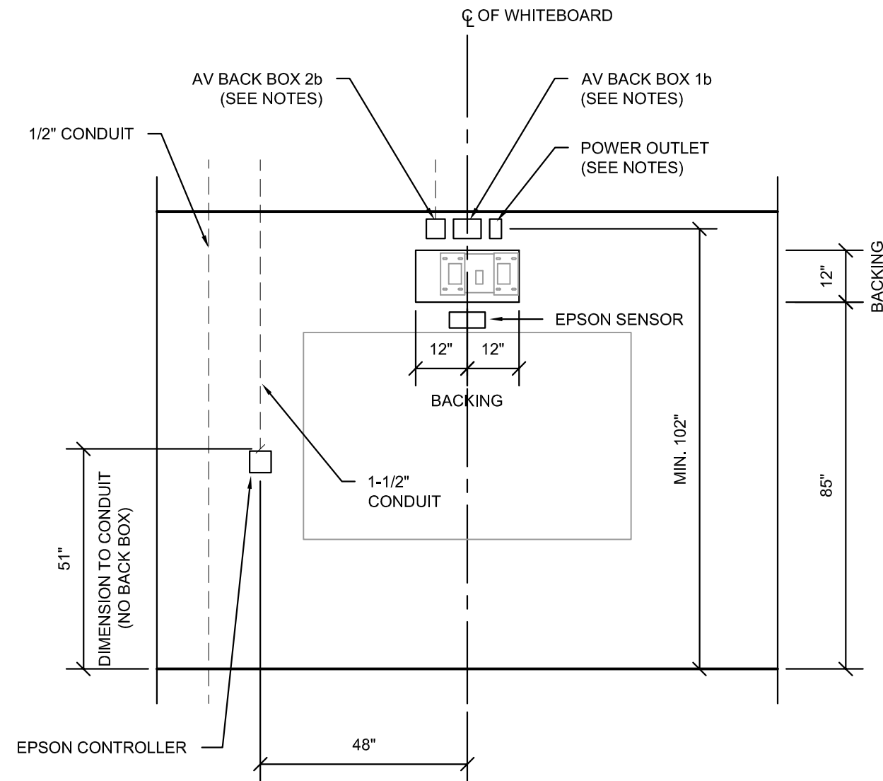
NORTH WALL - BACKING, BACK BOX & CONDUIT DETAILS
