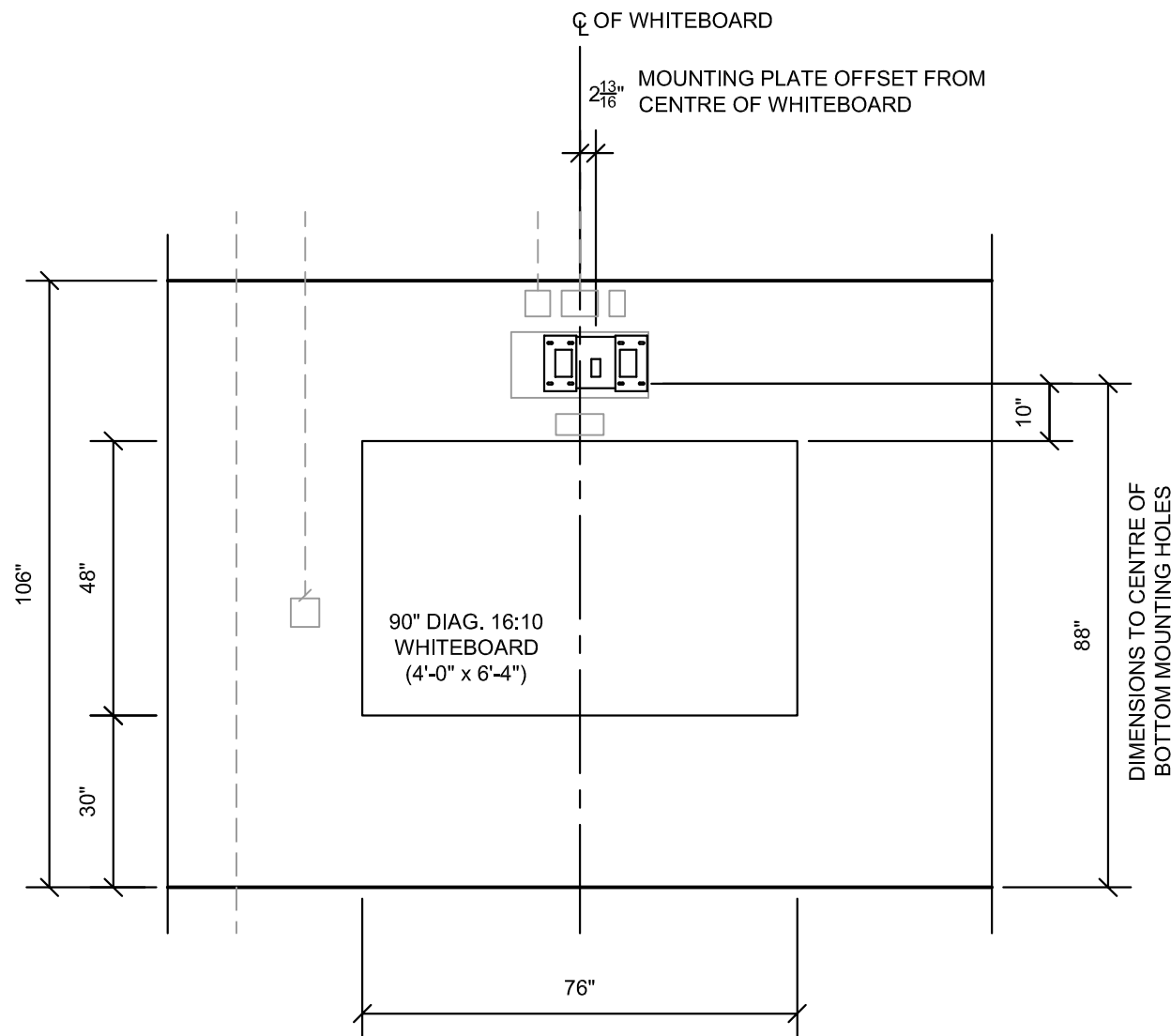
NORTH WALL - SHOWING WHITEBOARD & WALL MOUNT DIMENSIONS
