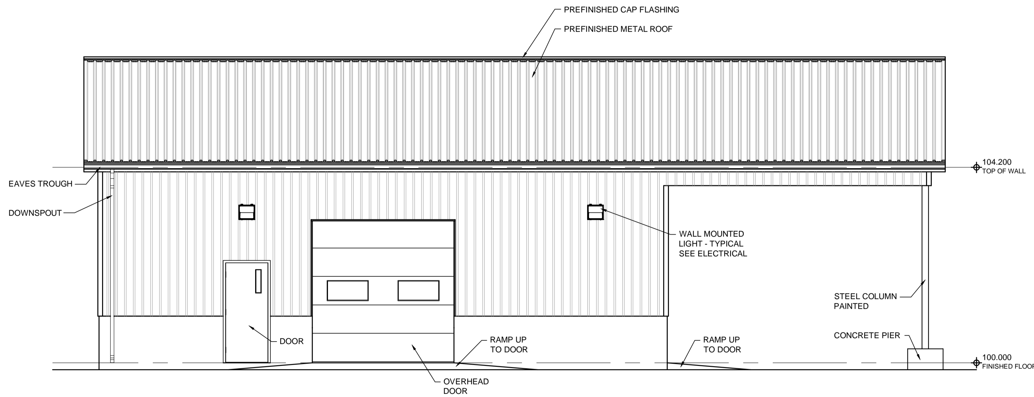
SOUTH ELEVATION 1:50
