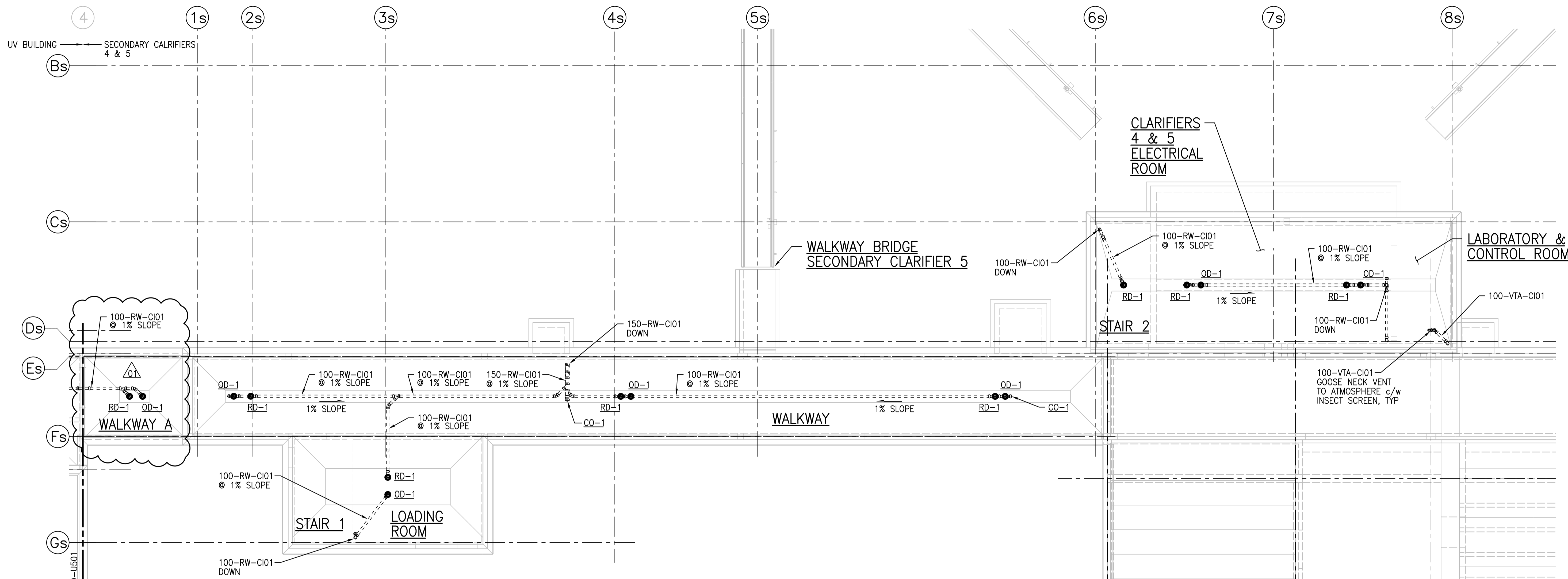
ROOF PLAN 1:100
