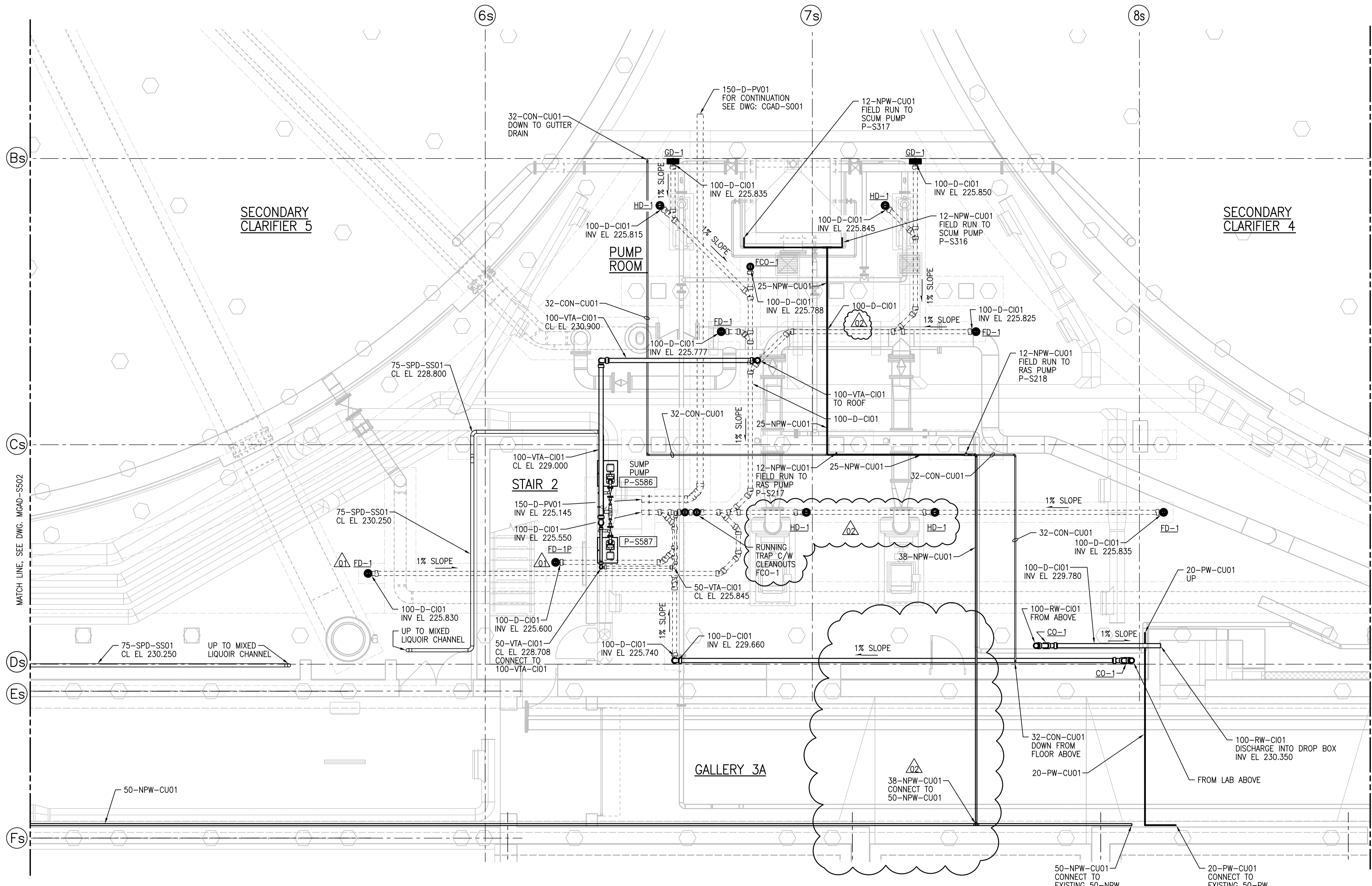
BASEMENT PLAN - PART B 1:50
