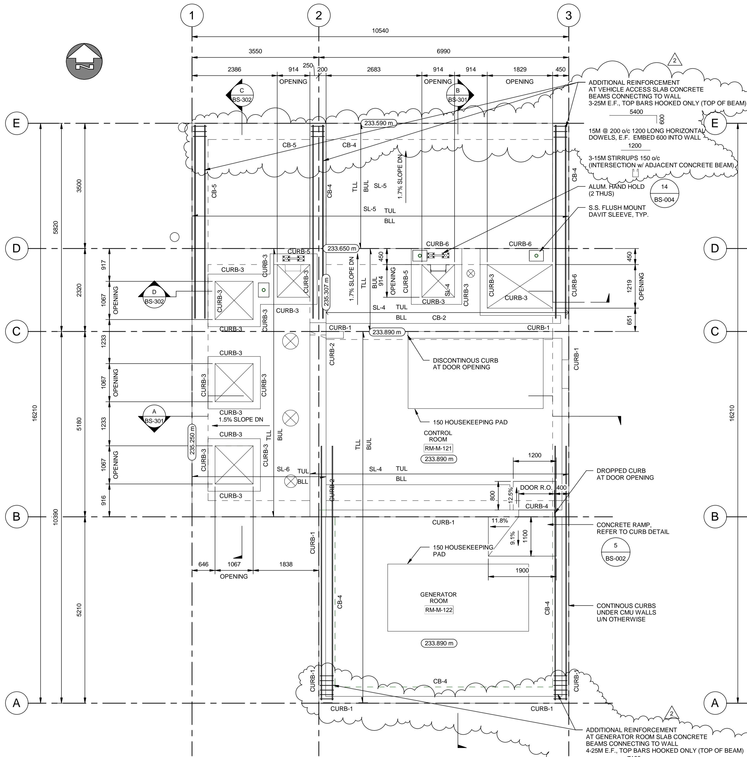
1 | MAIN LEVEL - CURBS & SLABS BS-103 SCALE: 1: 50
