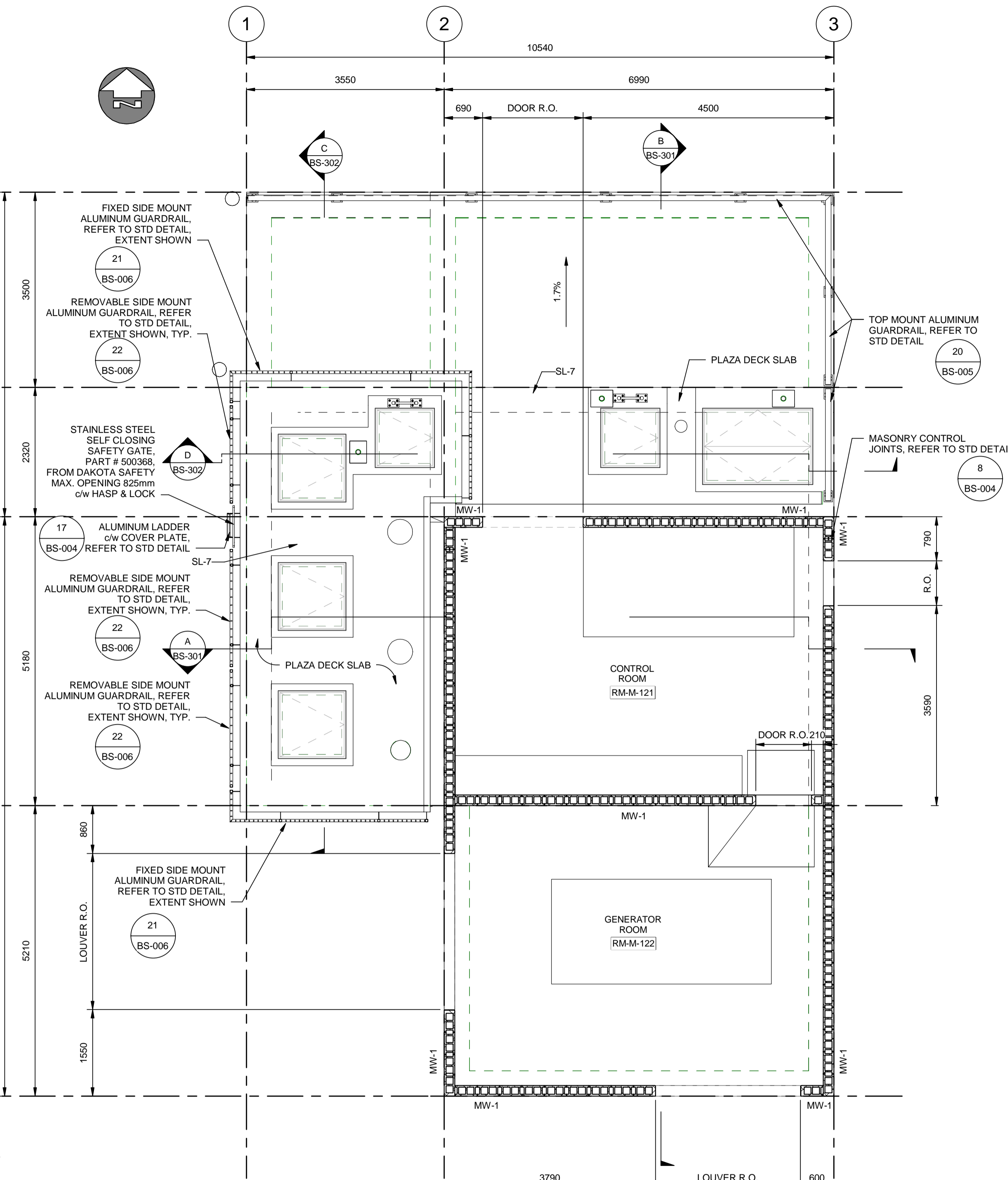
2 | MAIN LEVEL - WALLS BS-103 SCALE: 1: 50
