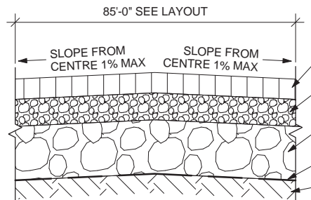
2 HOCKEY RINK PAVING SECTION 1 : 20
