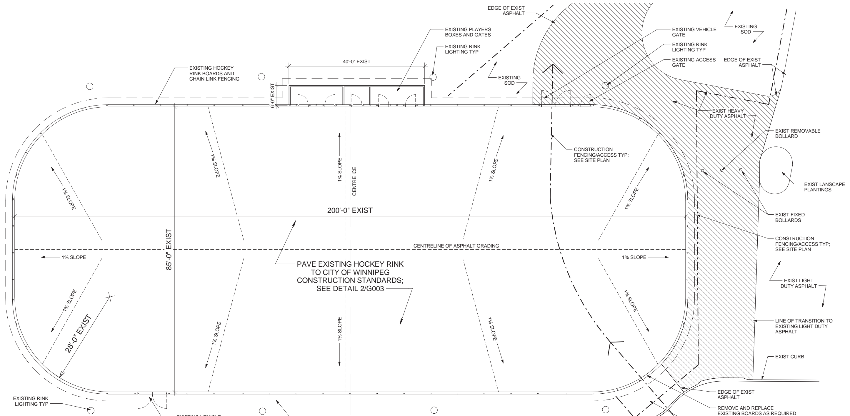
1 OUTDOOR HOCKEY RINK LAYOUT PLAN 1 : 200
