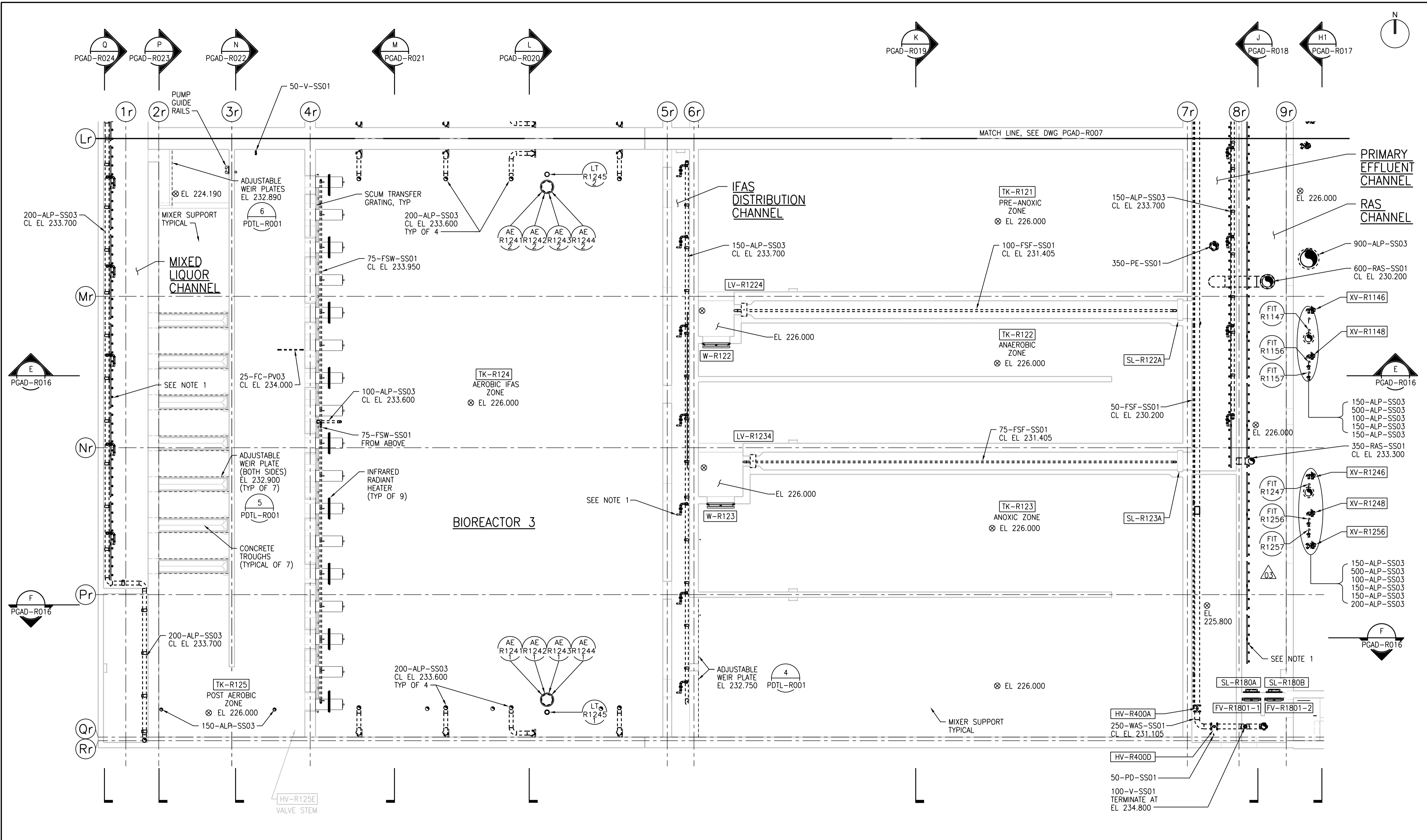
UPPER LEVEL PLAN - PART C 1:100
