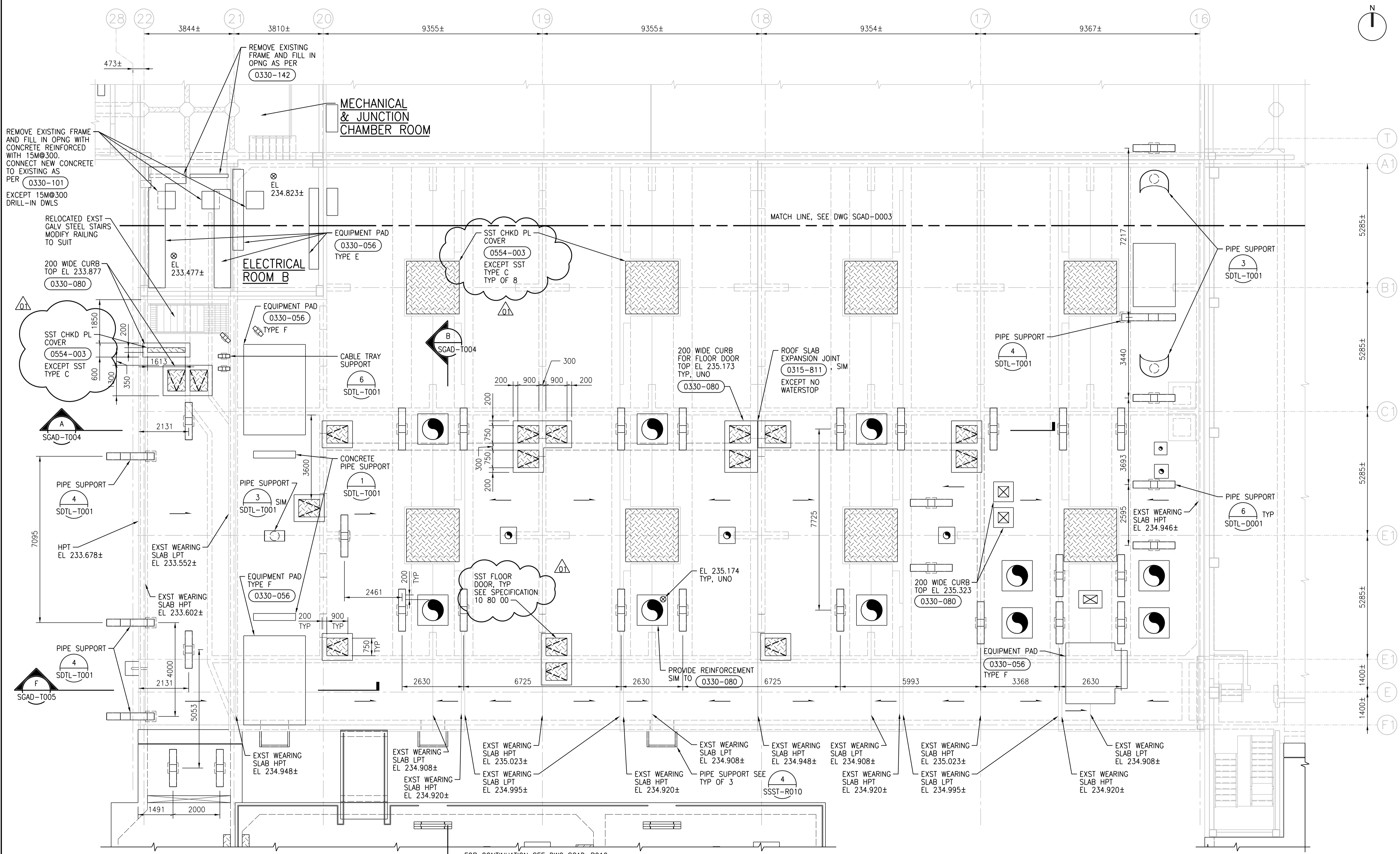
ROOF PLAN 1:75
