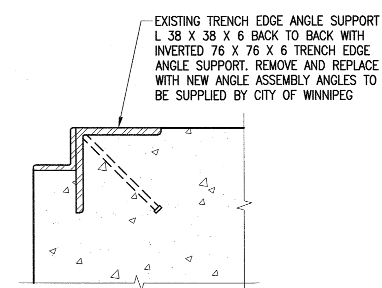
5 HYDRAULIC TRENCH SECTION S2.2 S4.2 1:20
