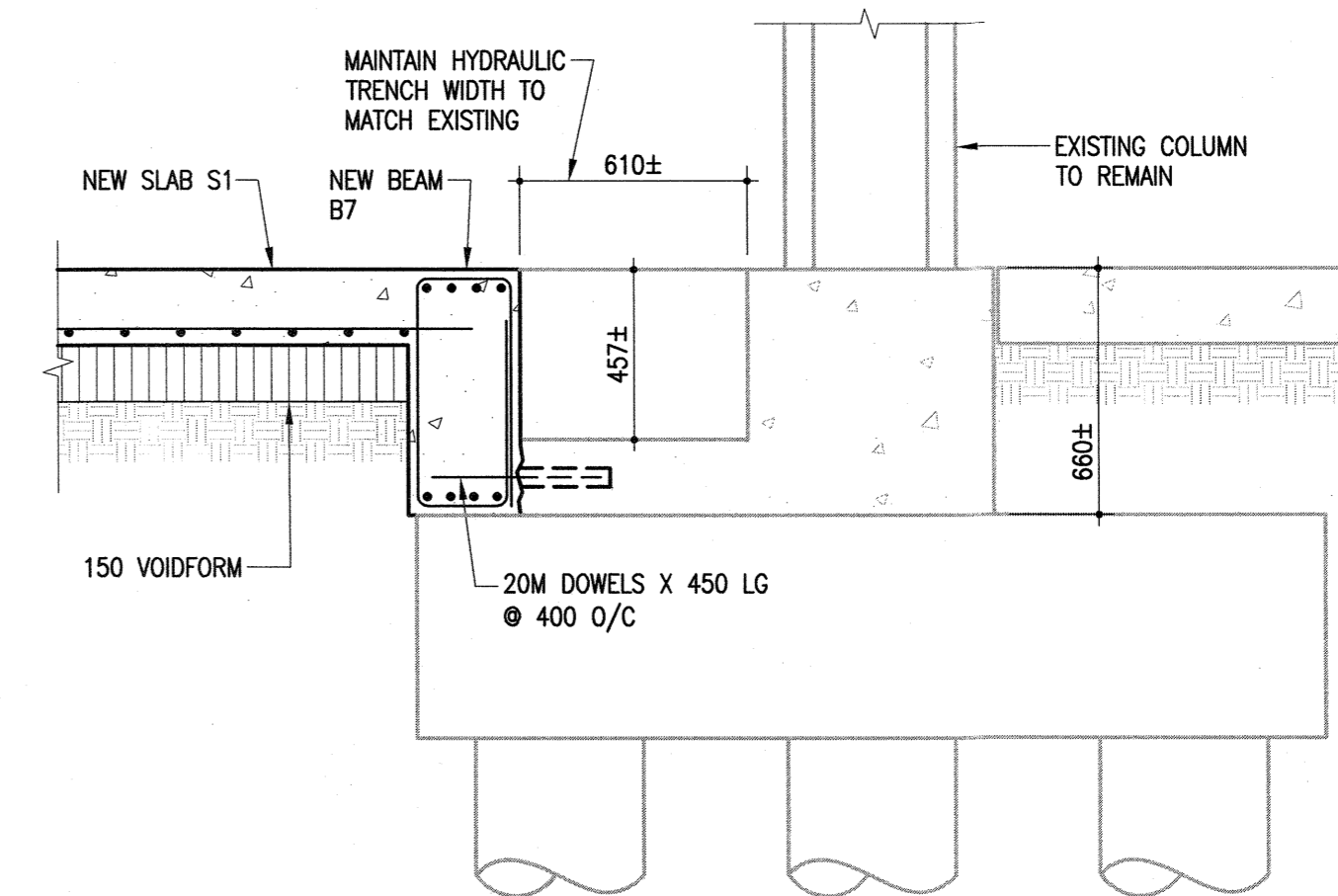
5 HYDRAULIC TRENCH SECTION S2.2 S4.2 1:20
