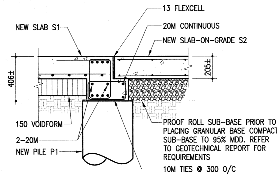
3 JOINT SECTION S2.2 S4.2 1:20
