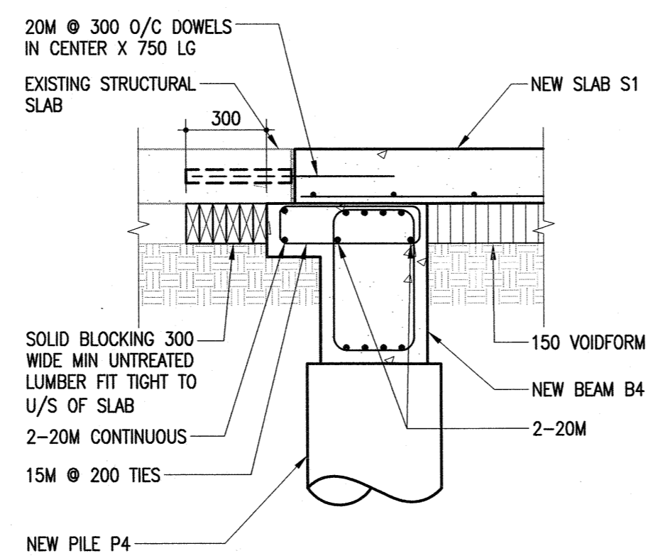
6 NEW - EXIST JOINT SECTION S2.2 S4.2 1:20
