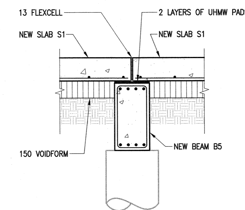
4 EXPANSION JOINT SECTION S2.2 S4.2 1:20
