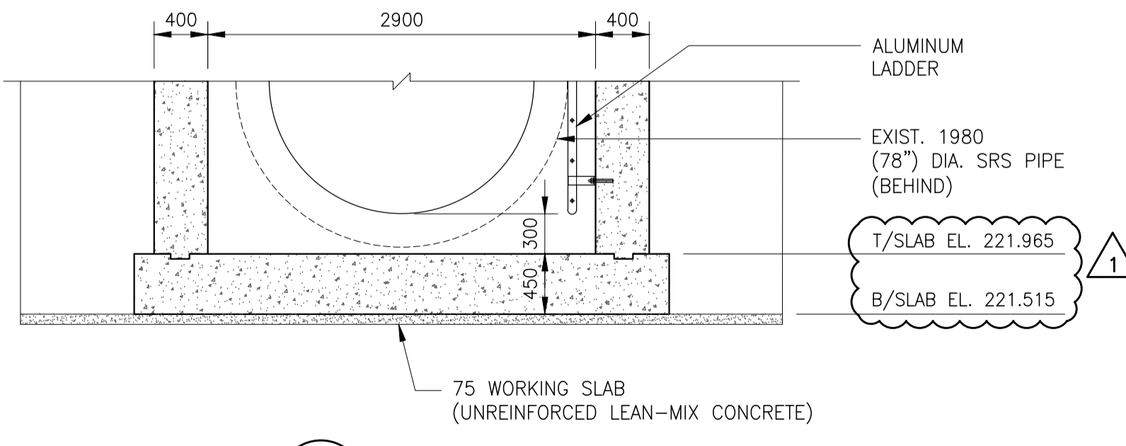
D SECTION SCALE:1:40
