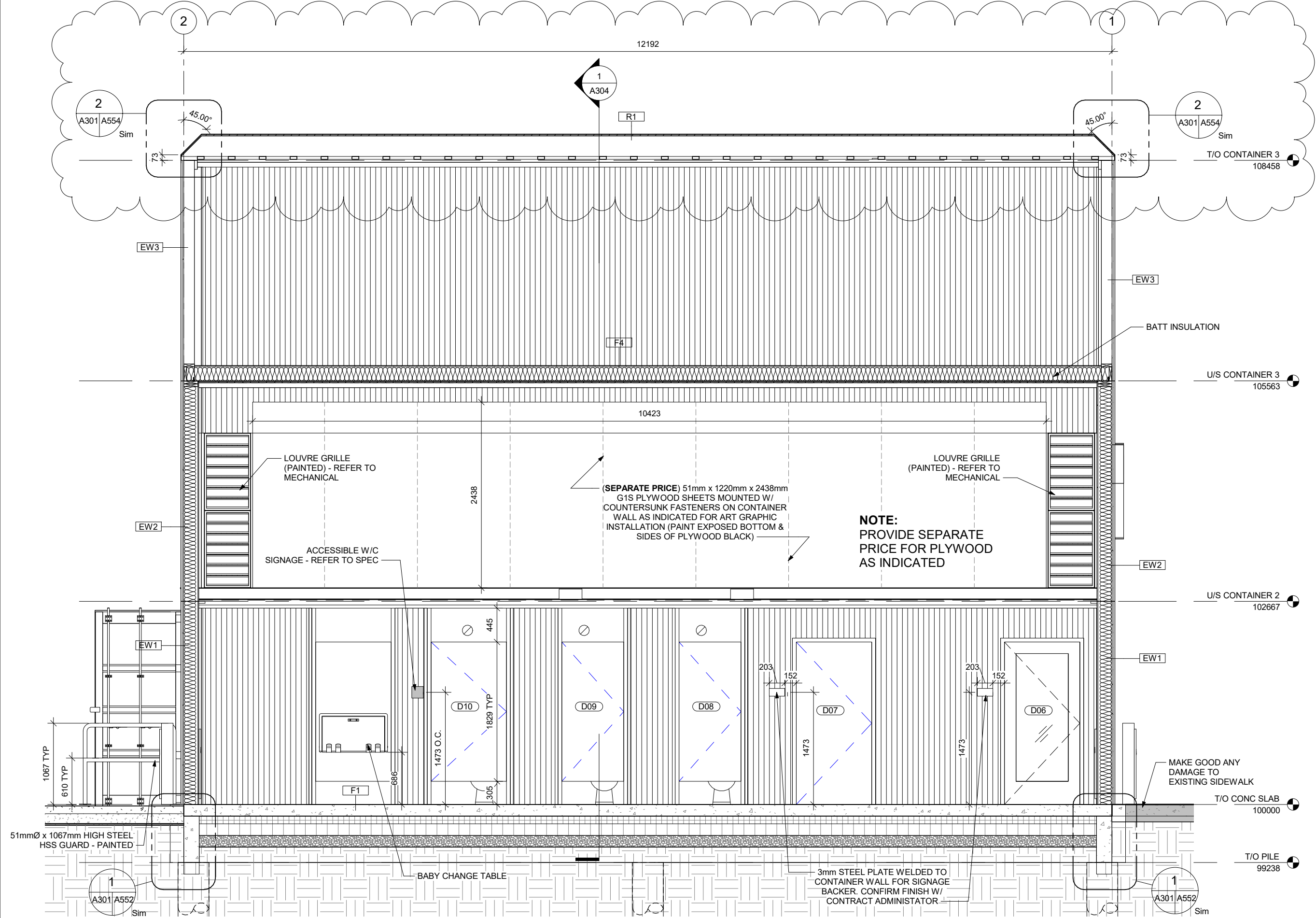
1 BUILDING SECTION 2 1 : 48
