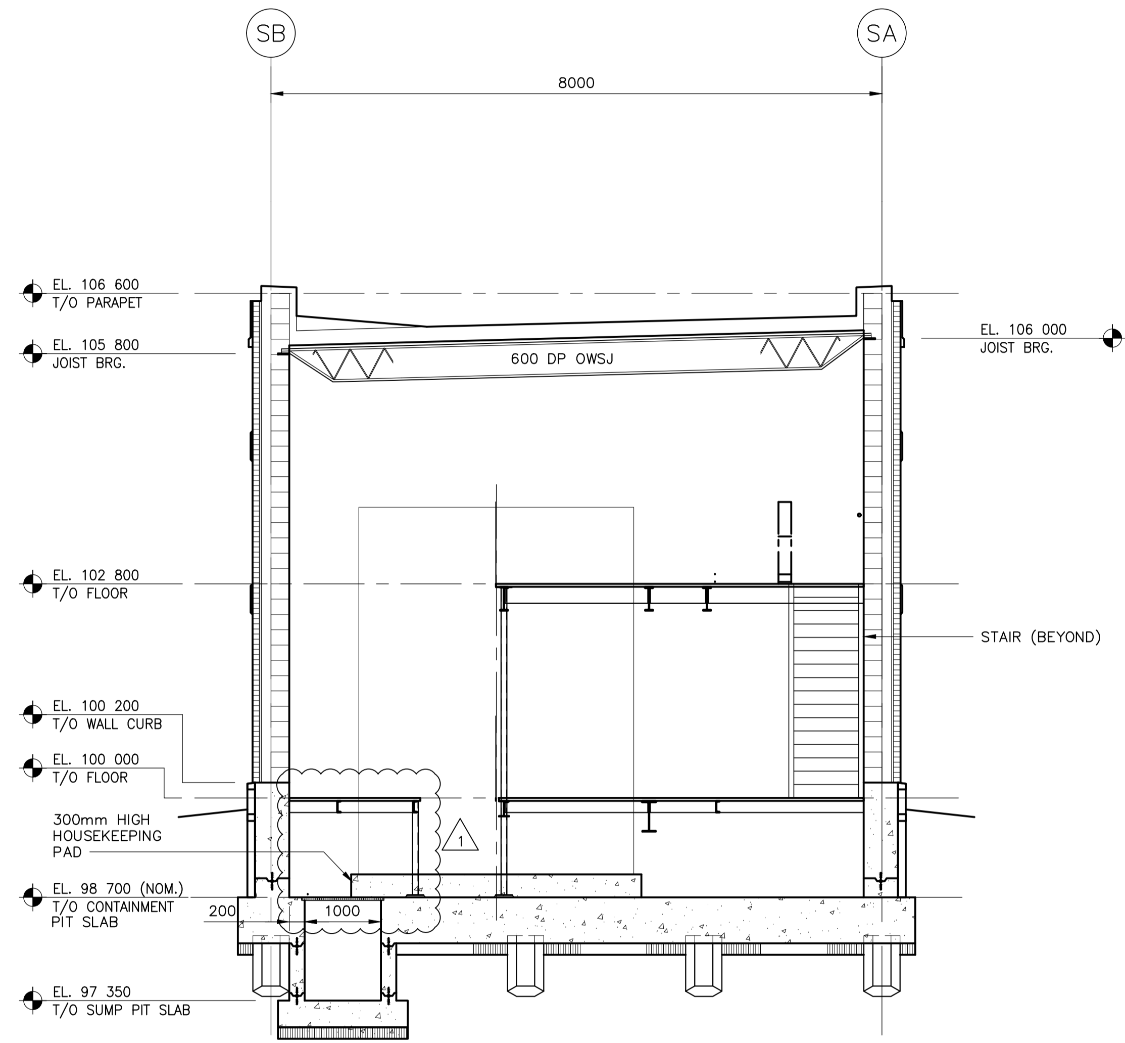
A SECTION - LOOKING WEST REF. 1 SCALE: 1:50
