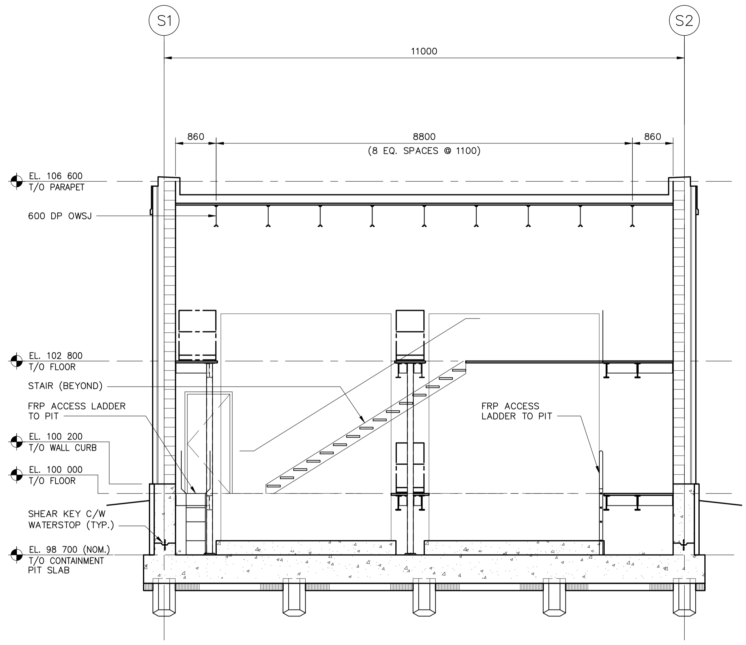
B SECTION - LOOKING NORTH REF. 1 SCALE: 1:50
