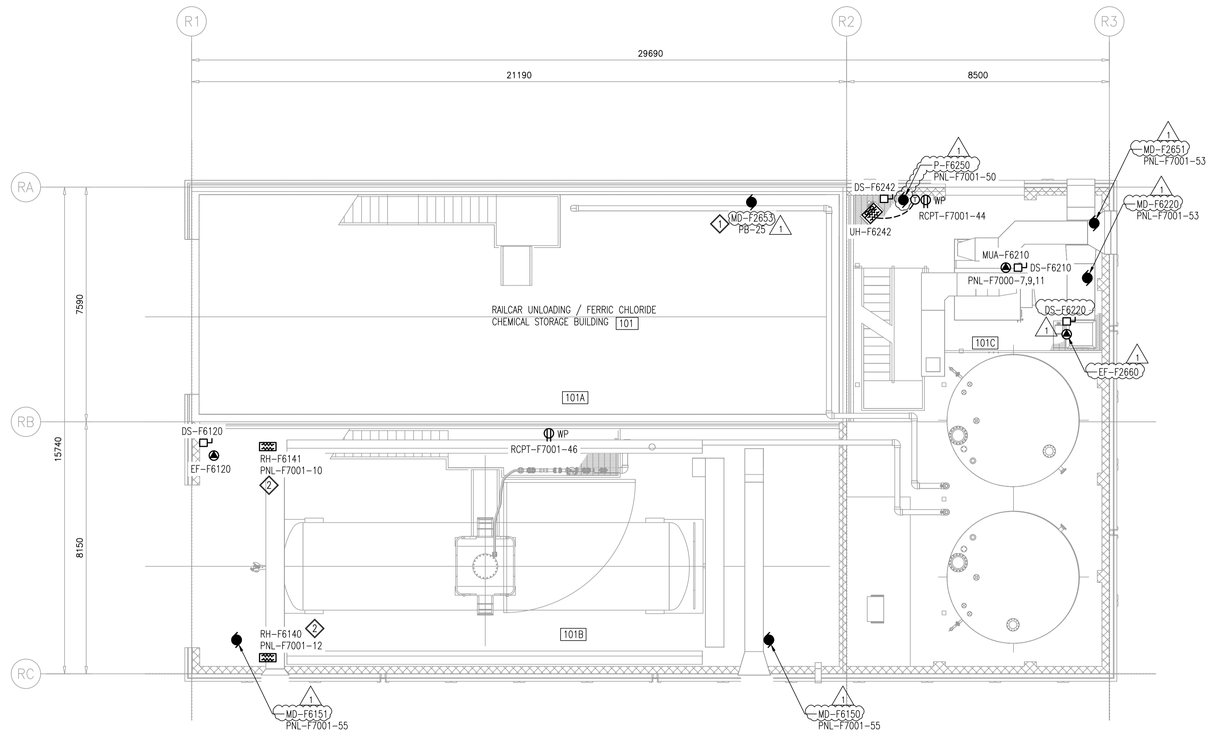
A PLAN - PLATFORM 1 SCALE: 1:75mm
