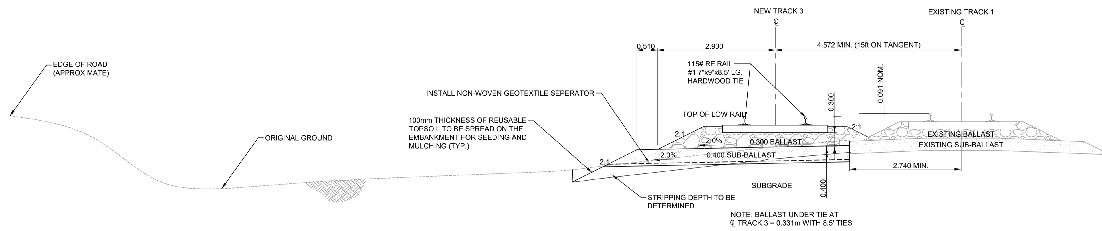
TYPICAL - TRACK 3 SECTION 1:50
