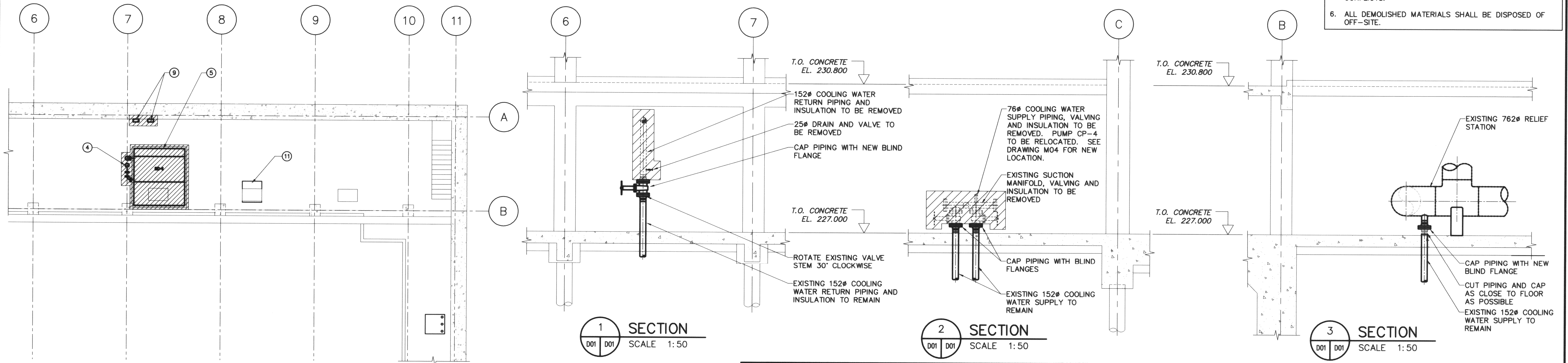
PARTIAL PLAN ABOVE EL. 232.450m SCALE: 1:100
