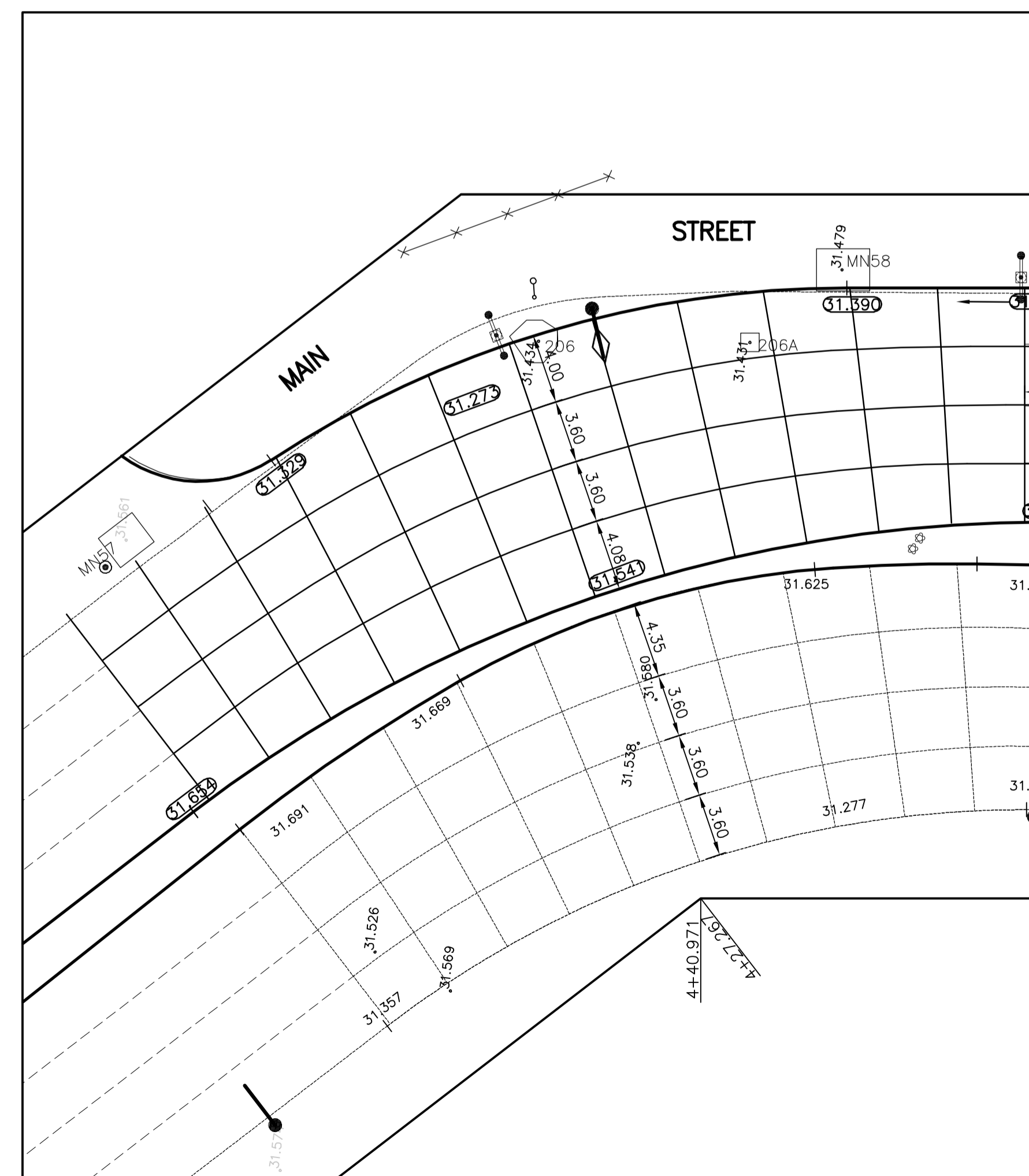
JOINT DETAIL AT STA. 4+40
