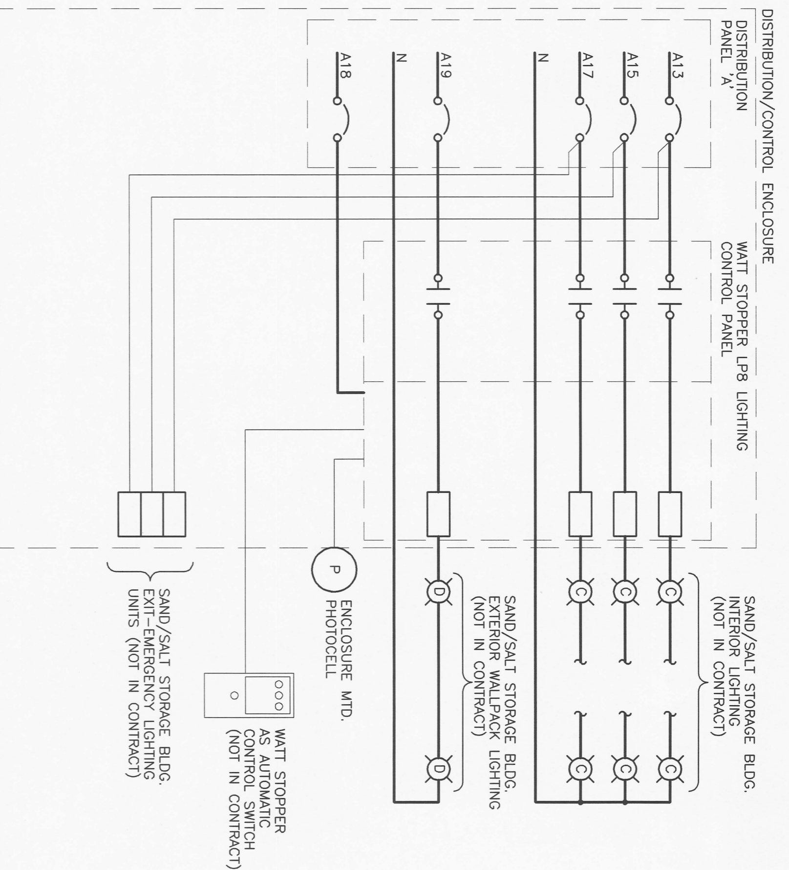
B LIGHTING CONTROL SCHEMATIC N.T.S.
