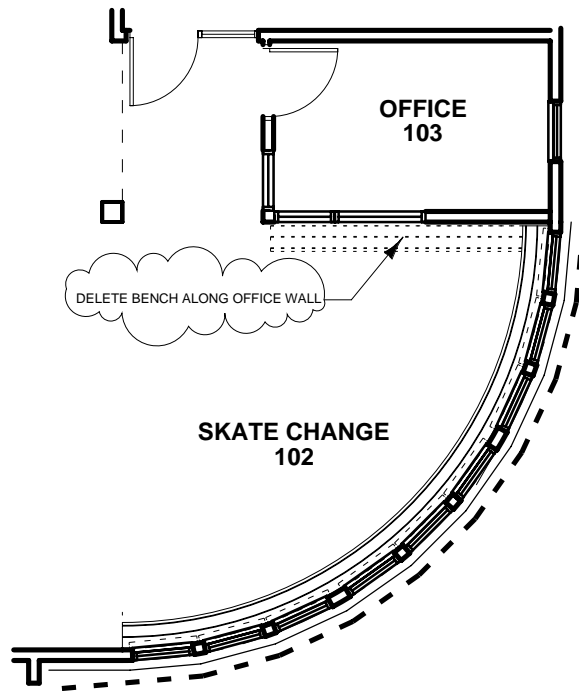
PARTIAL PLAN FOR SKATECHANGE 102 REFER TO FLOOR PLAN A2-1
