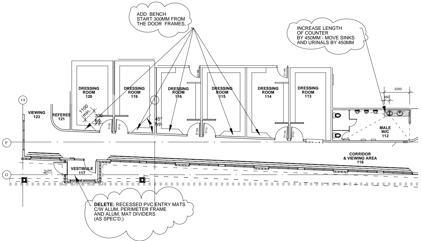
PARTIAL PLAN FOR CORRIDOR 118, MALE W/C 112 & VESTIBULE 117 REFER TO FLOOR PLAN A2-1
