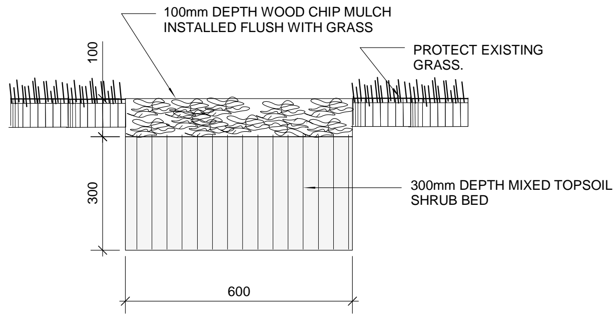
2 TYPICAL SHRUB BED SECTION L6 Scale: 1:10
