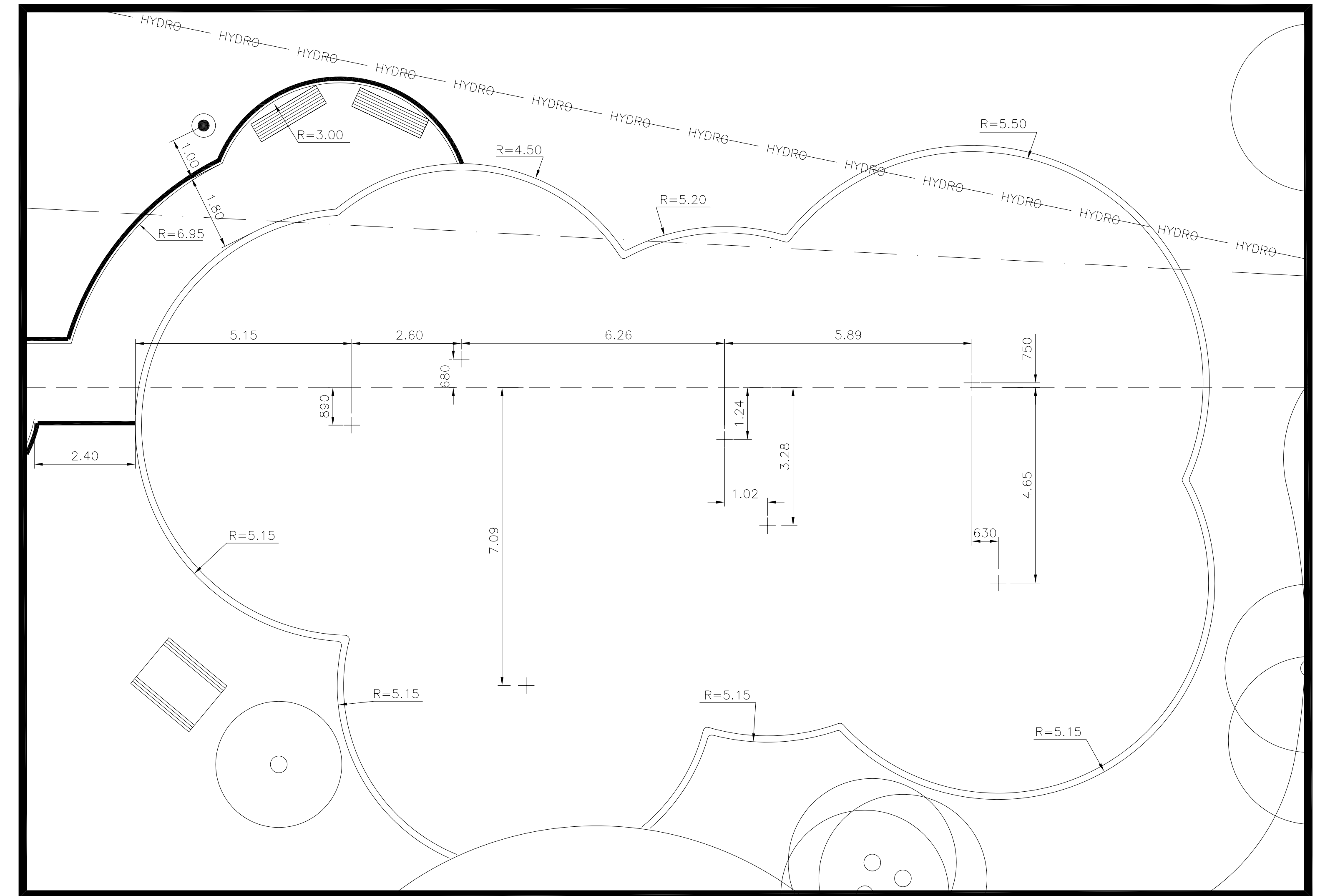
ENLARGEMENT 3: LAYOUT PLAN FOR PLAY AREA
