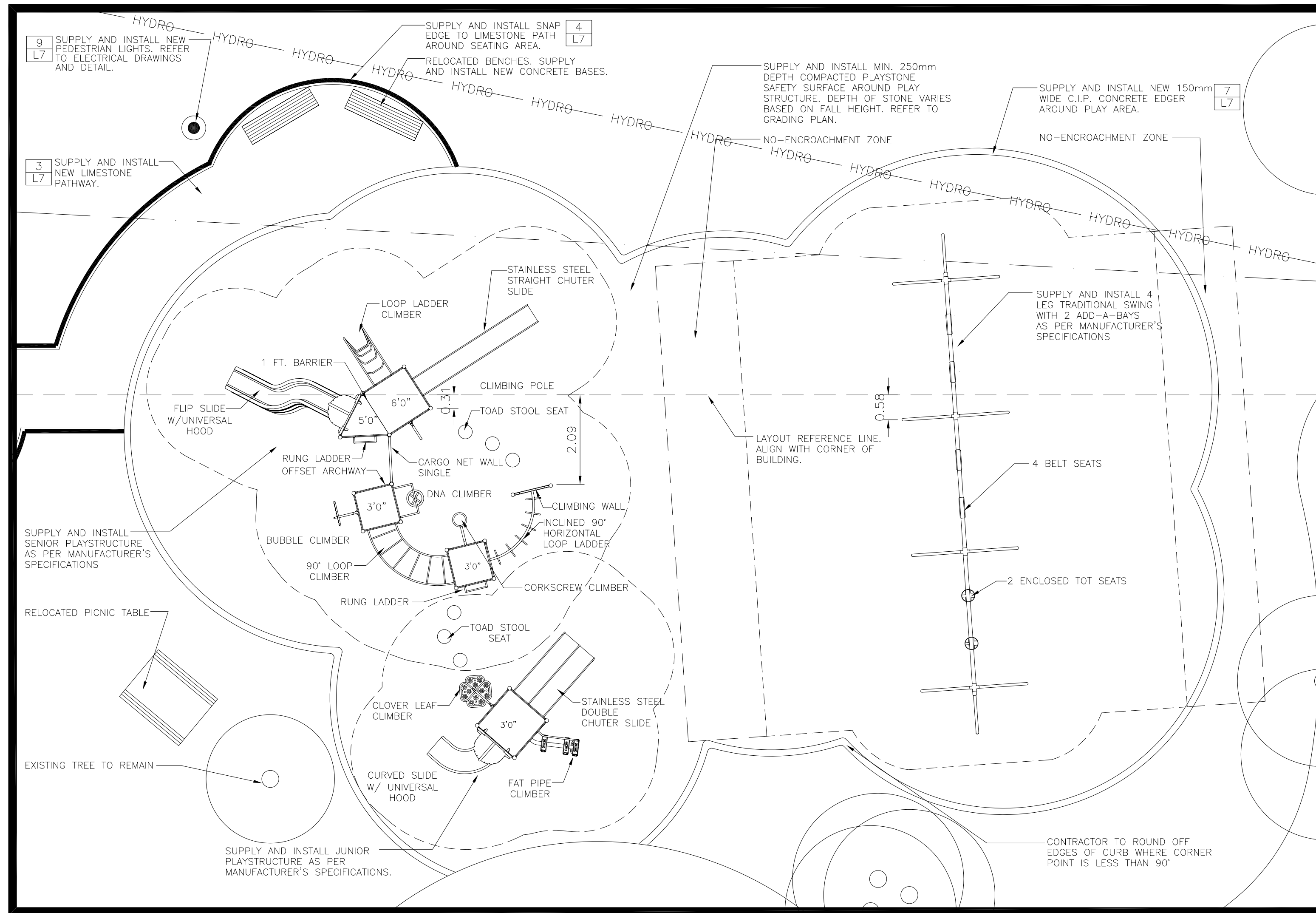
ENLARGEMENT 2: MATERIALS PLAN FOR PLAY AREA
