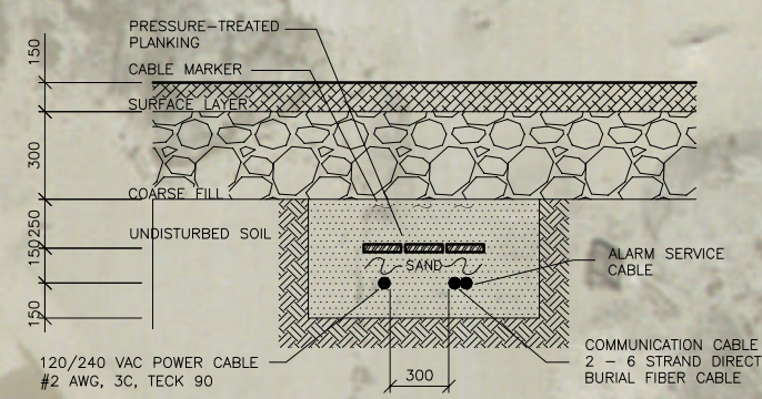
1 DIRECT-BURIED CABLES TRENCH DETAIL NTS
