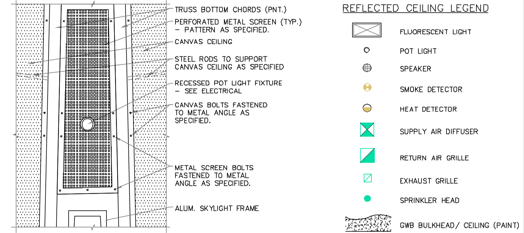
6 UNDER TRUSS DETAIL 1 : 20
