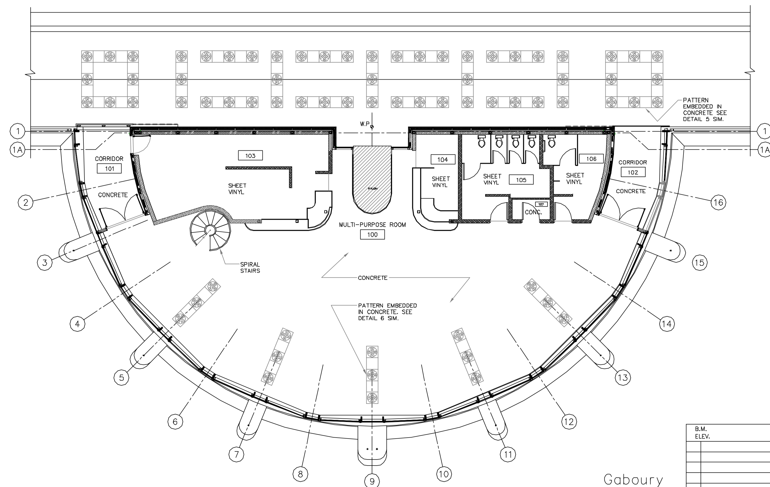
4 CENTRE PLAZA ENCLOSURE - FLOOR FINISH PLAN 1 : 100
