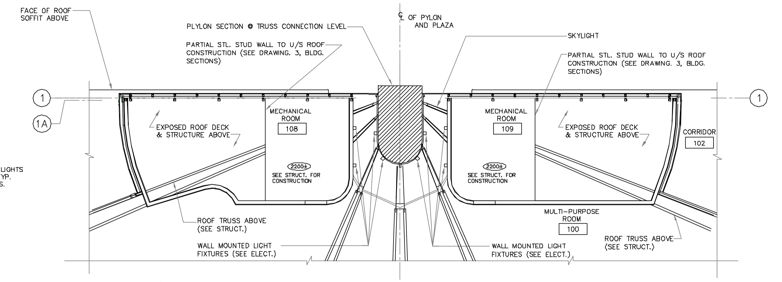
3 MECHANICAL ROOMS - REFLECTED CEILING PLAN 1 : 100
