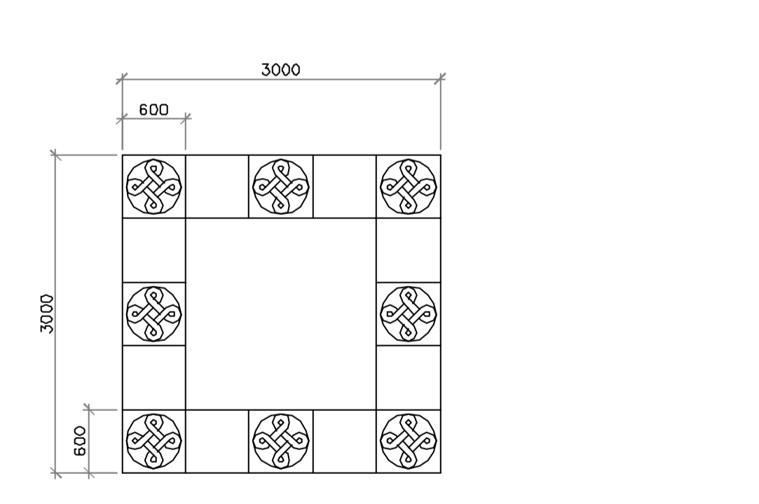
5 EXAMPLE OF CONCRETE MEDALLION 1 : 50
