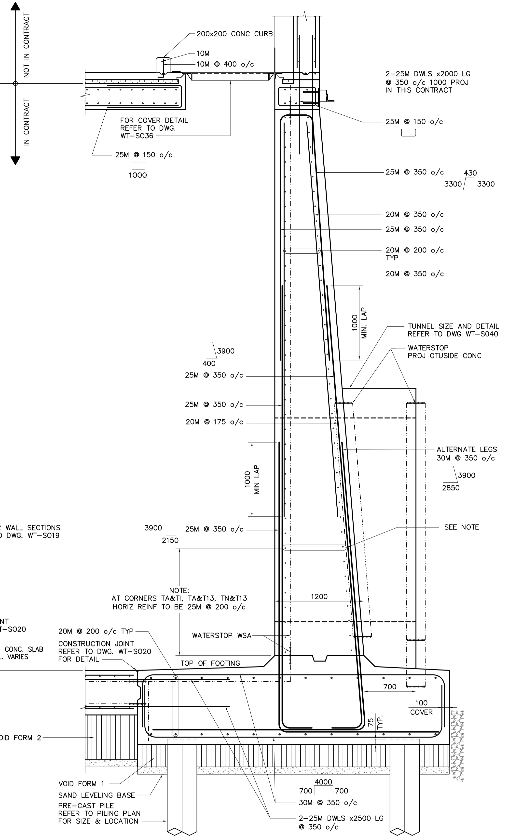
H DETAIL WT-S014 1:25
