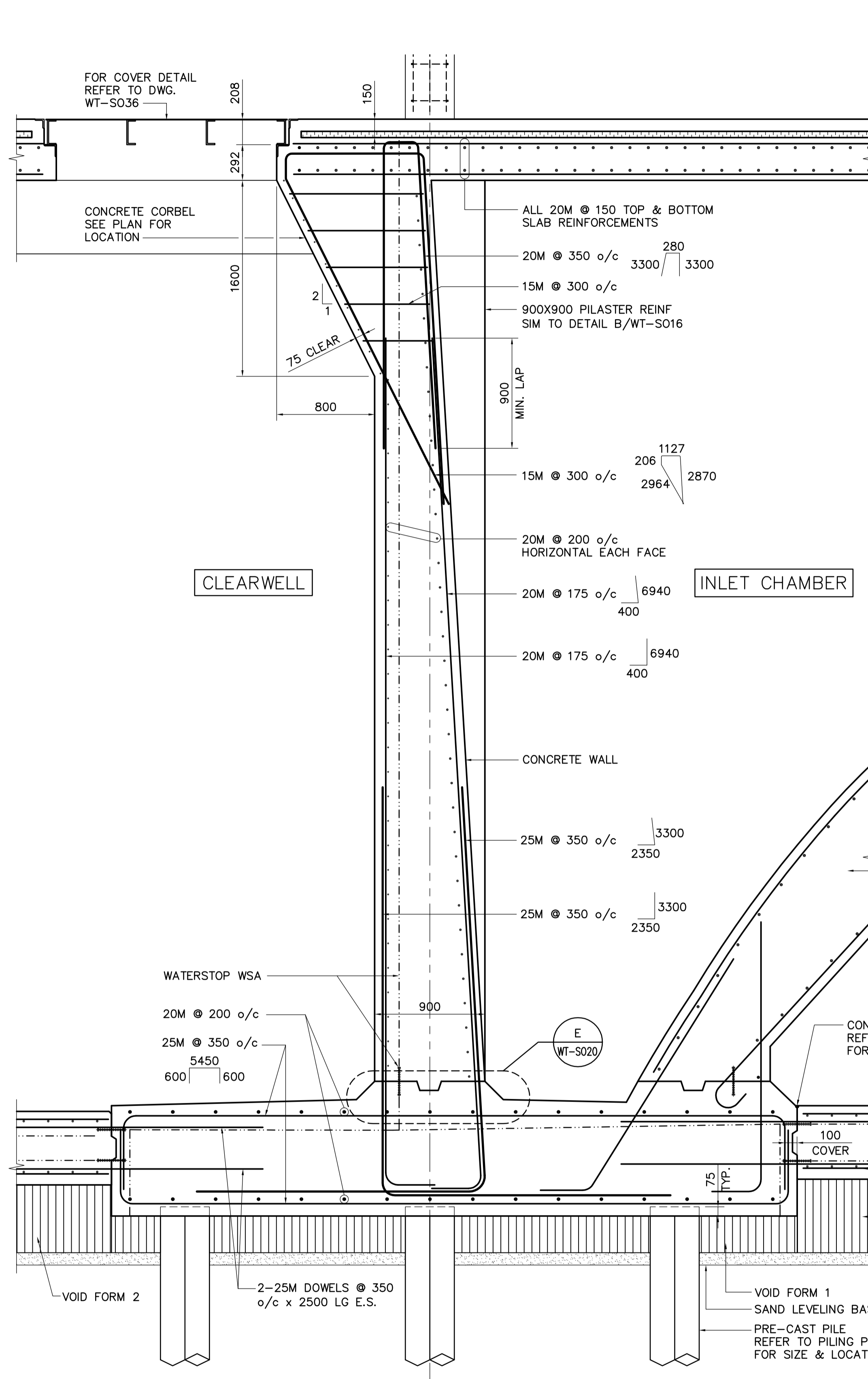
G DETAIL WT-S014 1:25
