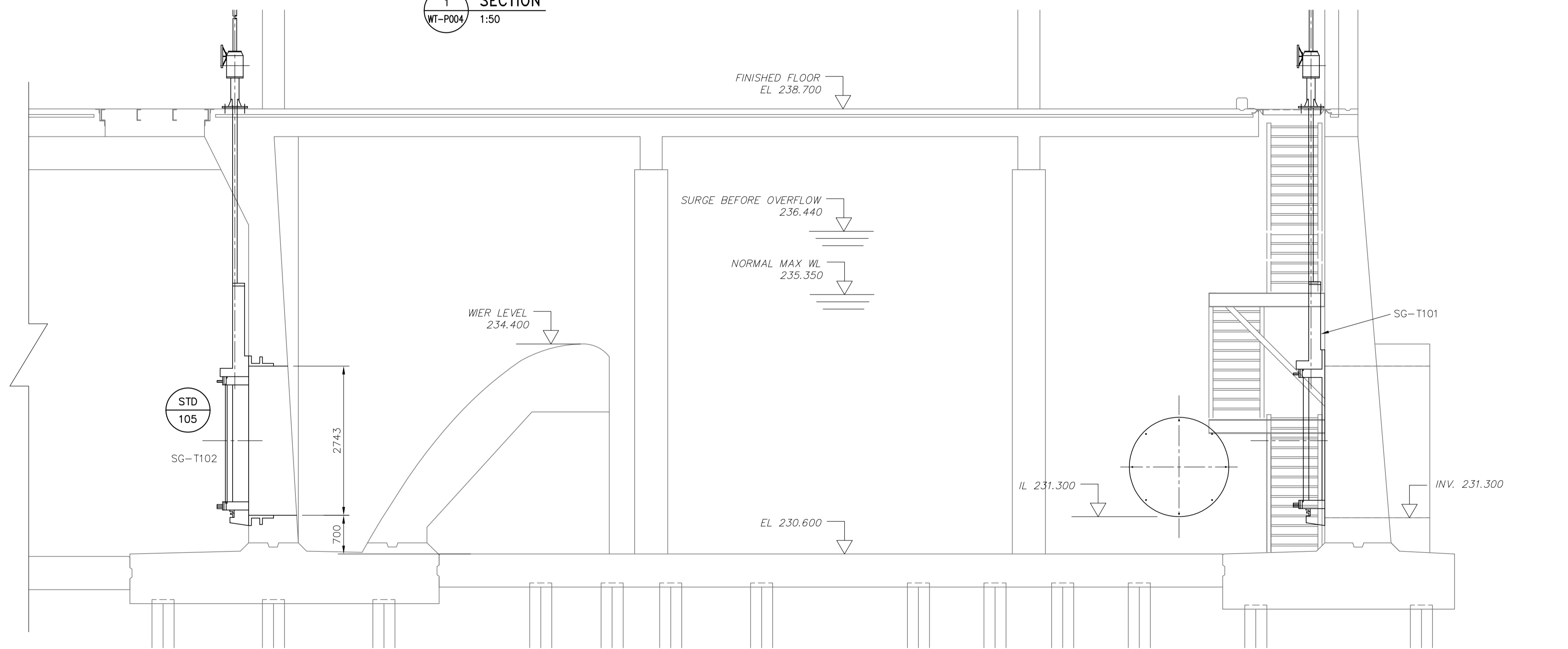
2 SECTION WT-P004 1:50
