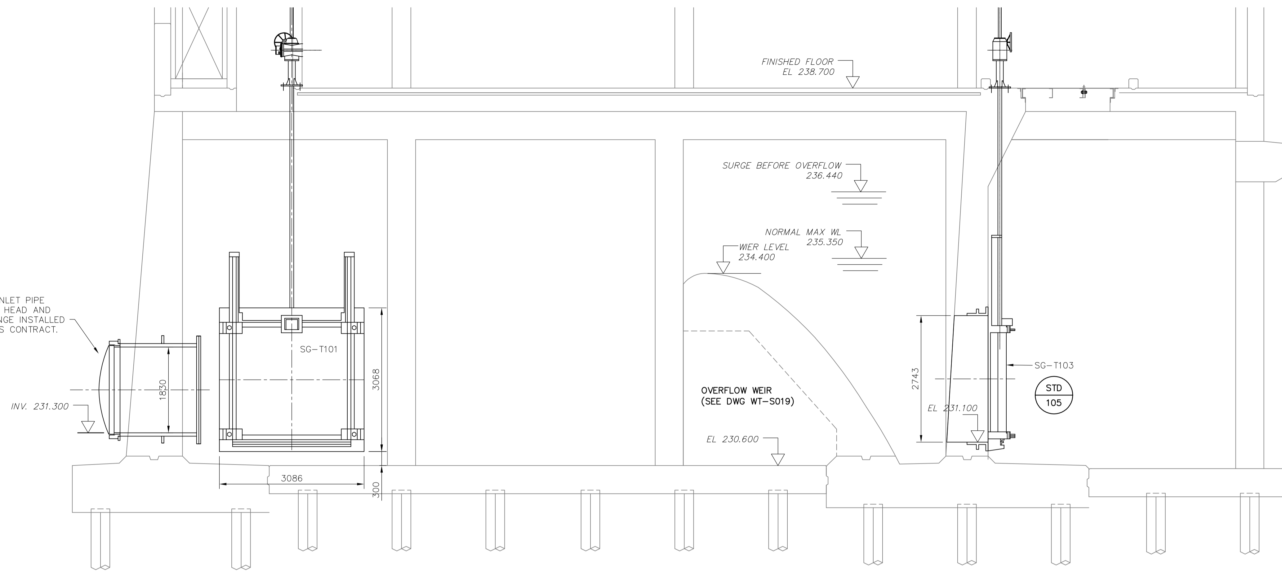
1 SECTION WT-P004 1:50
