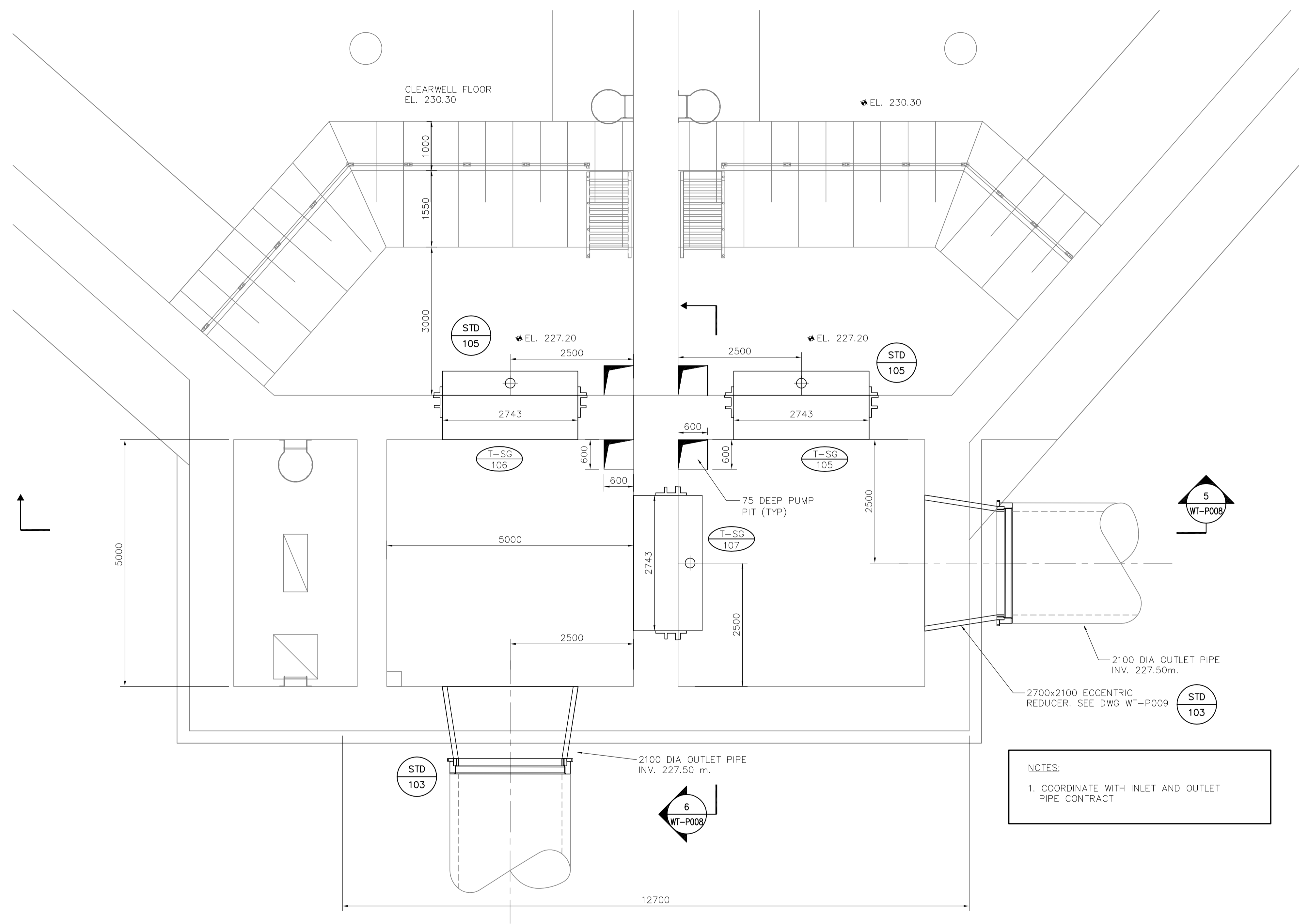
OUTLET BUILDING PLAN AT 230.30m 1:50
