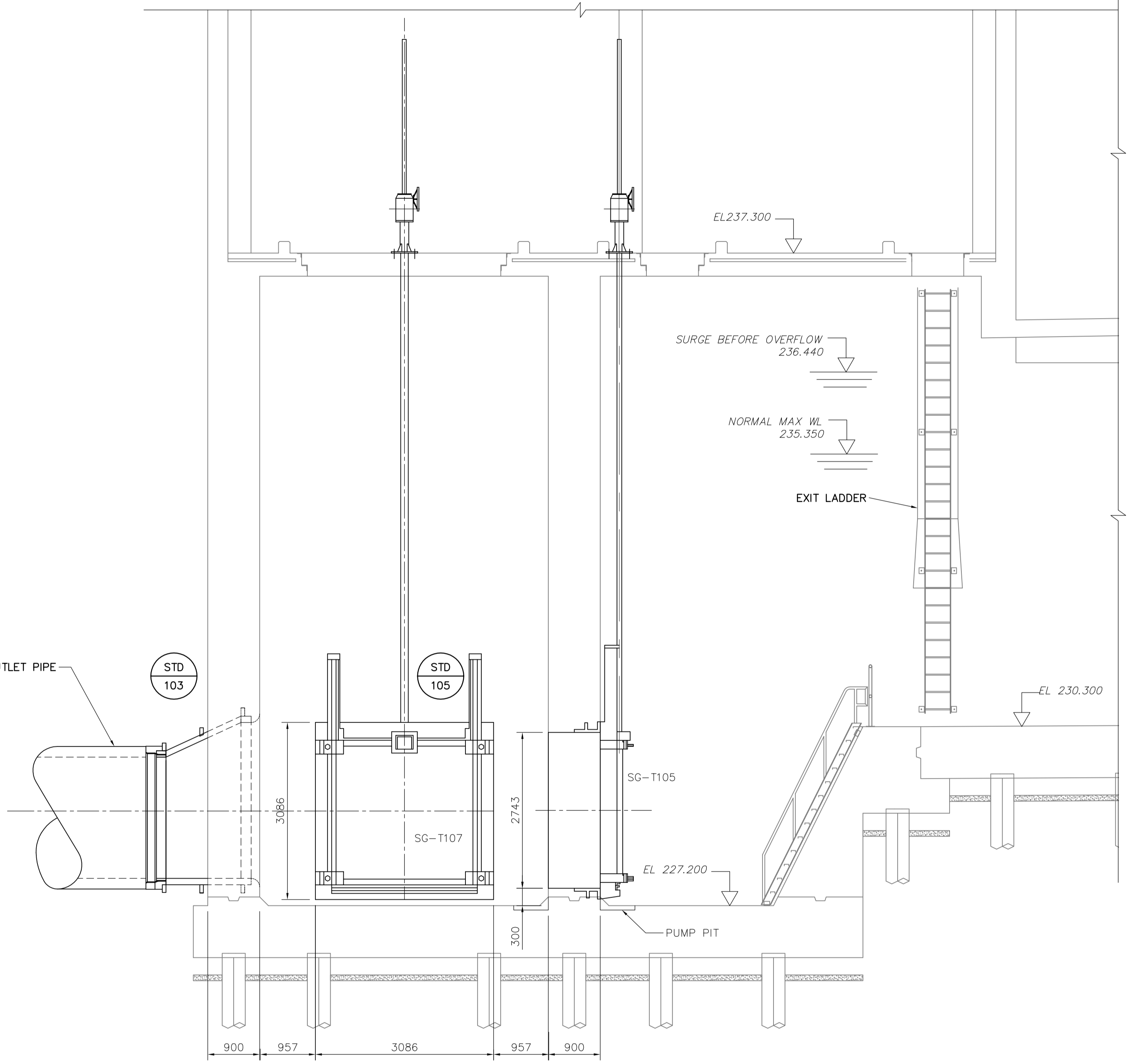
6 SECTION WT-P007 1:50
