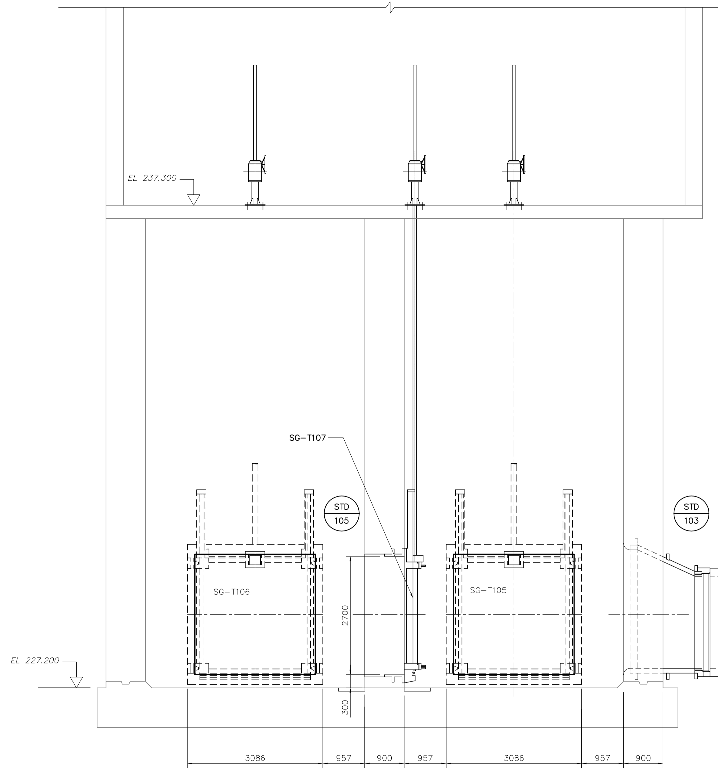
5 SECTION WT-P007 1:50
