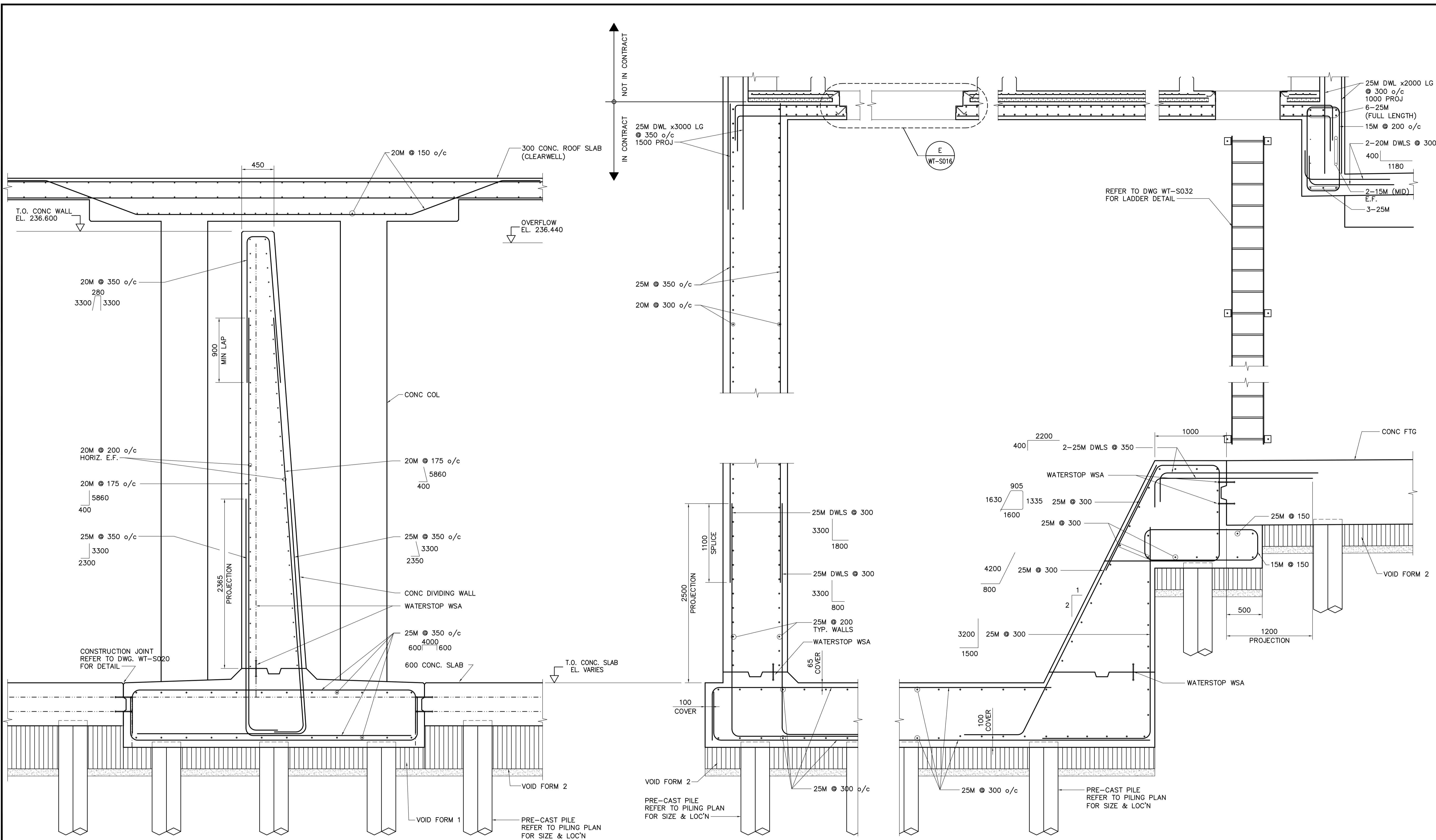
K DETAIL WT-S015 1:25
