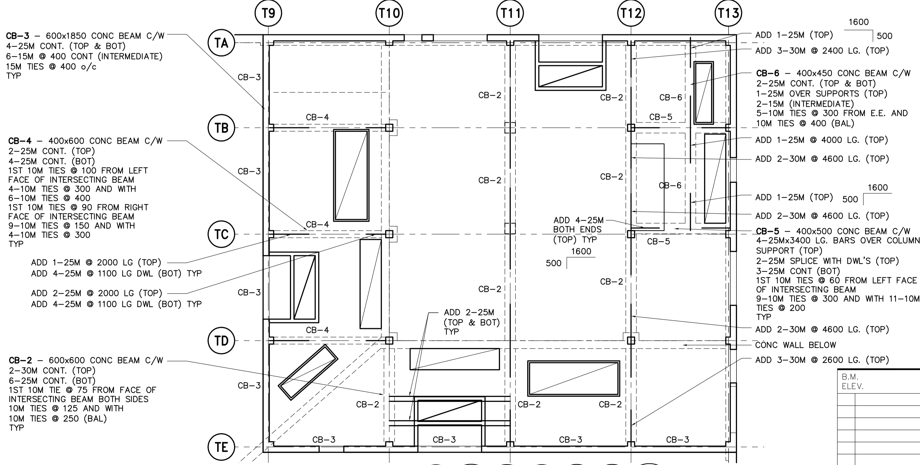
MAIN FLOOR BEAM REINFORCING PLAN N.T.S. ISSUED FOR STRUC SLAB REINF INFO ONLY
