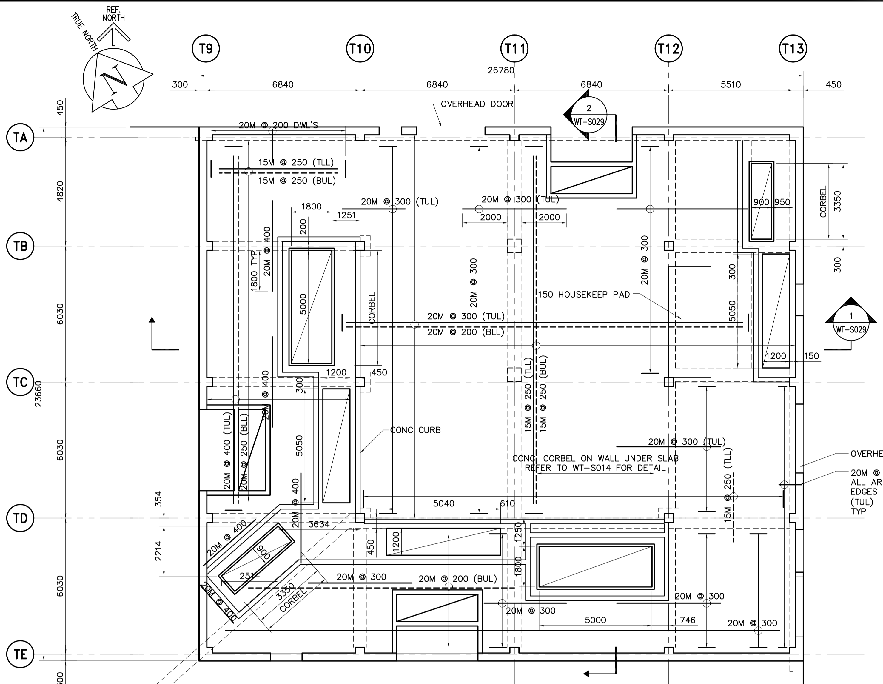
MAIN FLOOR FRAMING PLAN 1:100 ISSUED FOR FLOOR PENETRATION INFO ONLY
