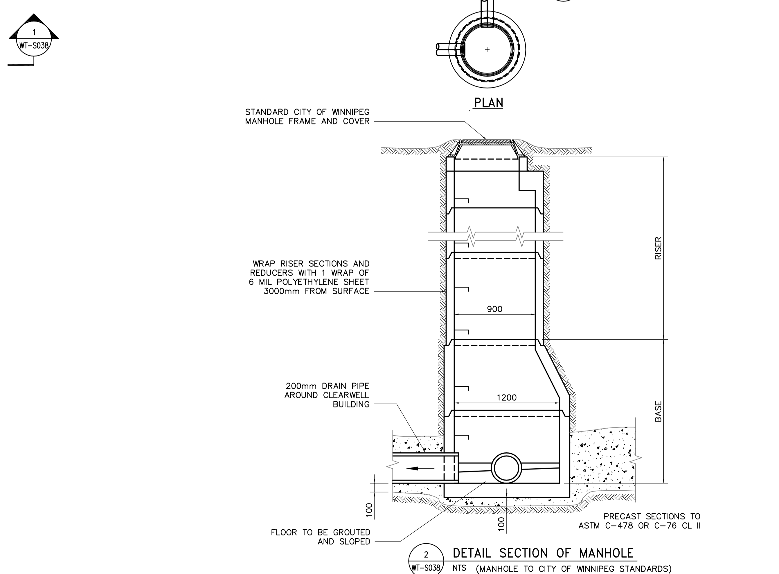
1 DETAIL 1:50
