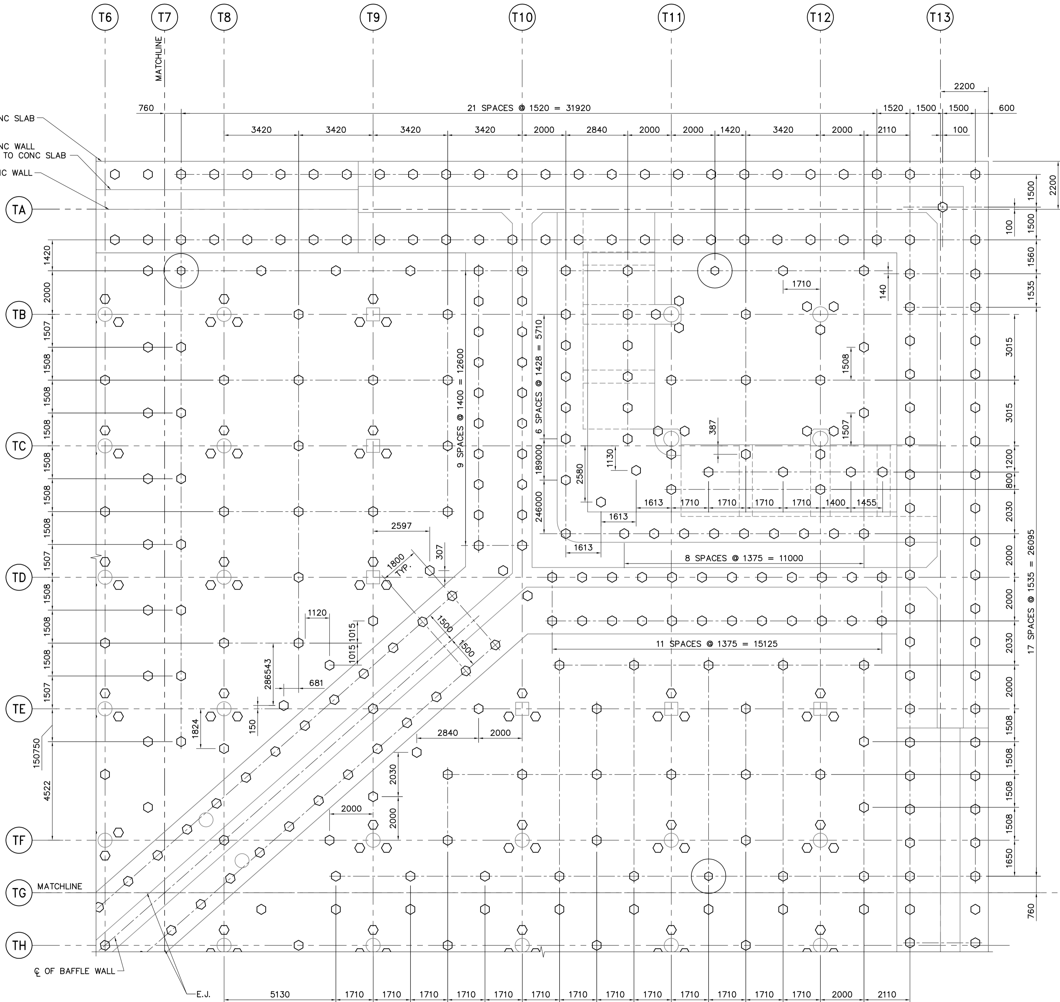
PARTIAL PILING PLAN 1:100
