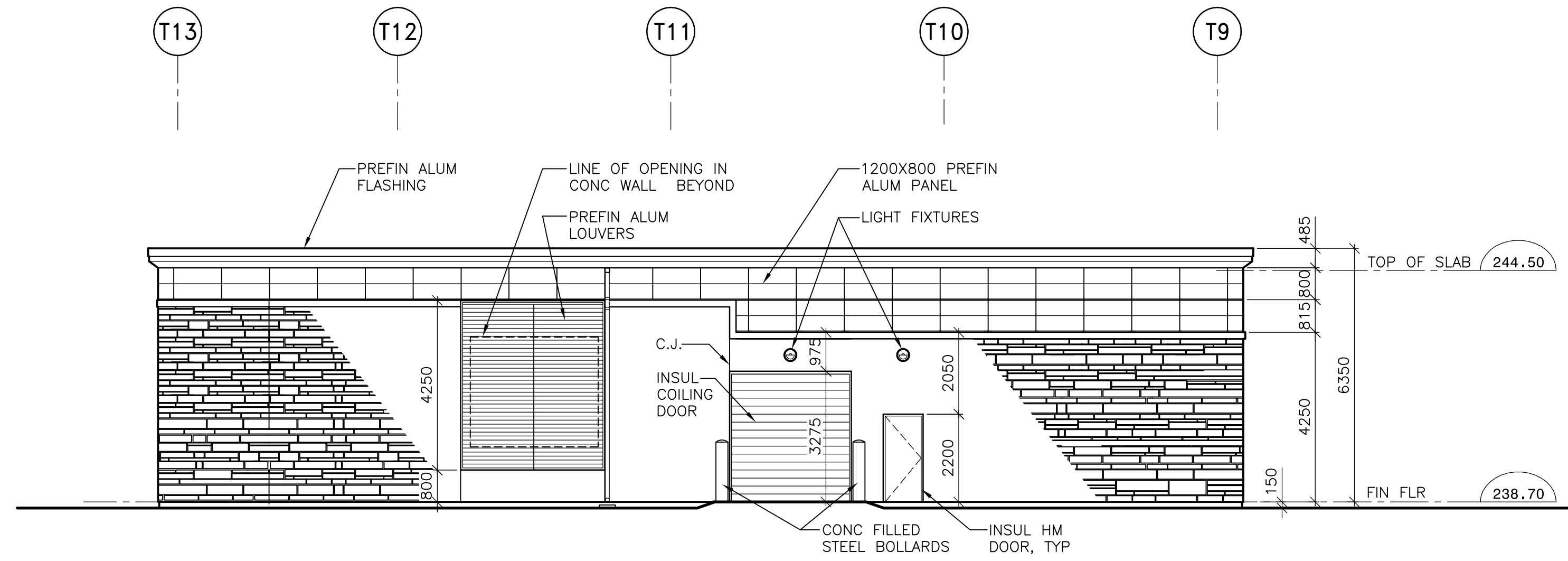
NORTH ELEVATION 1:100
