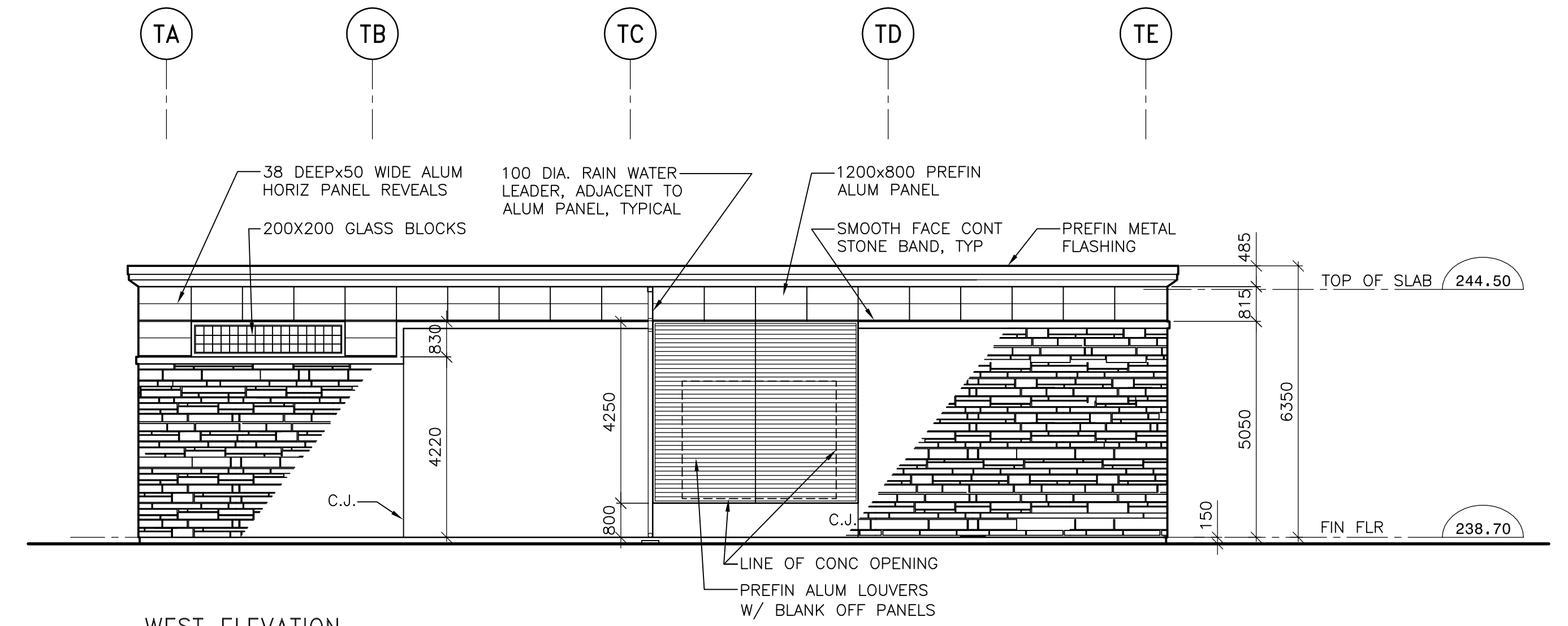
WEST ELEVATION 1:100
