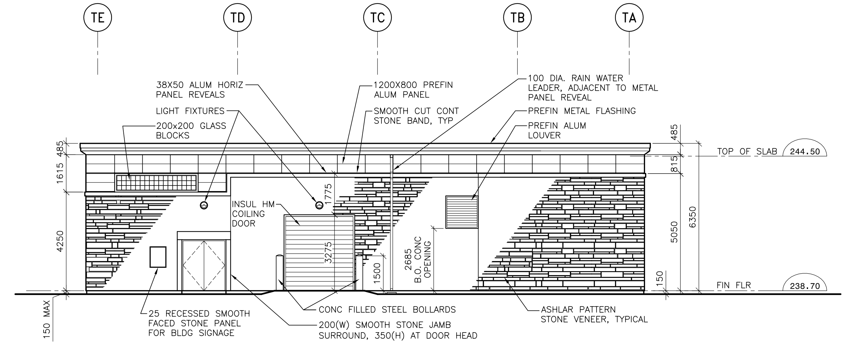
EAST ELEVATION 1:100
