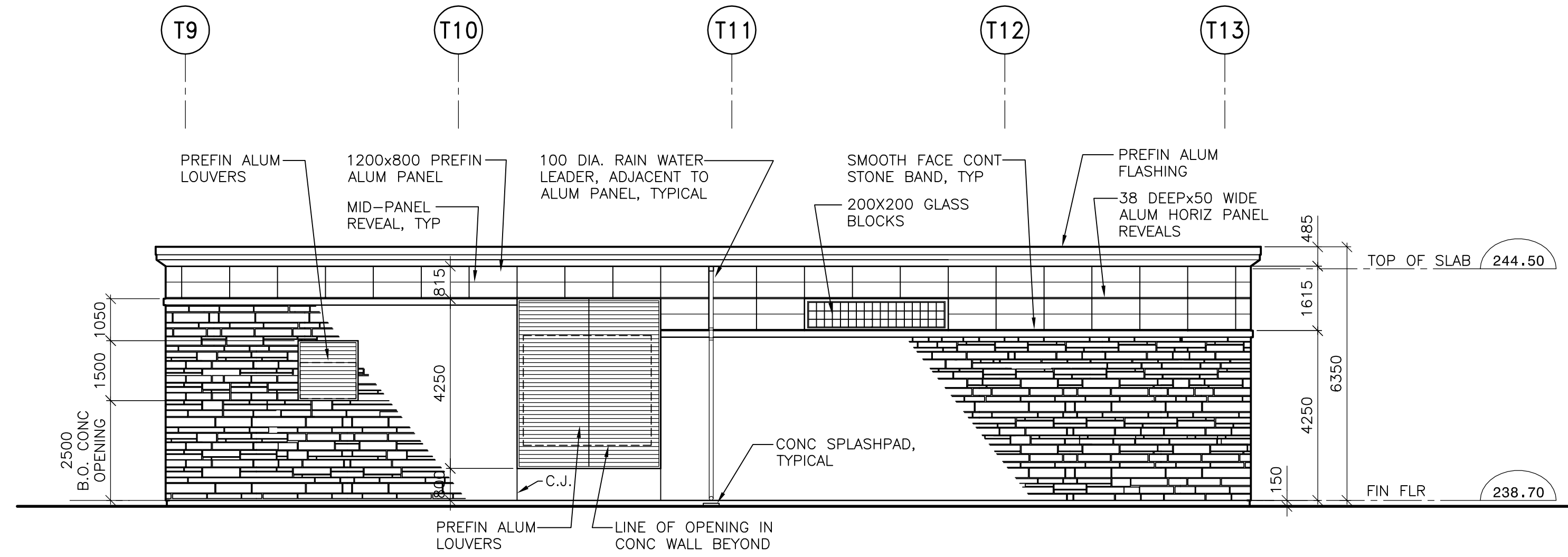
SOUTH ELEVATION 1:100
