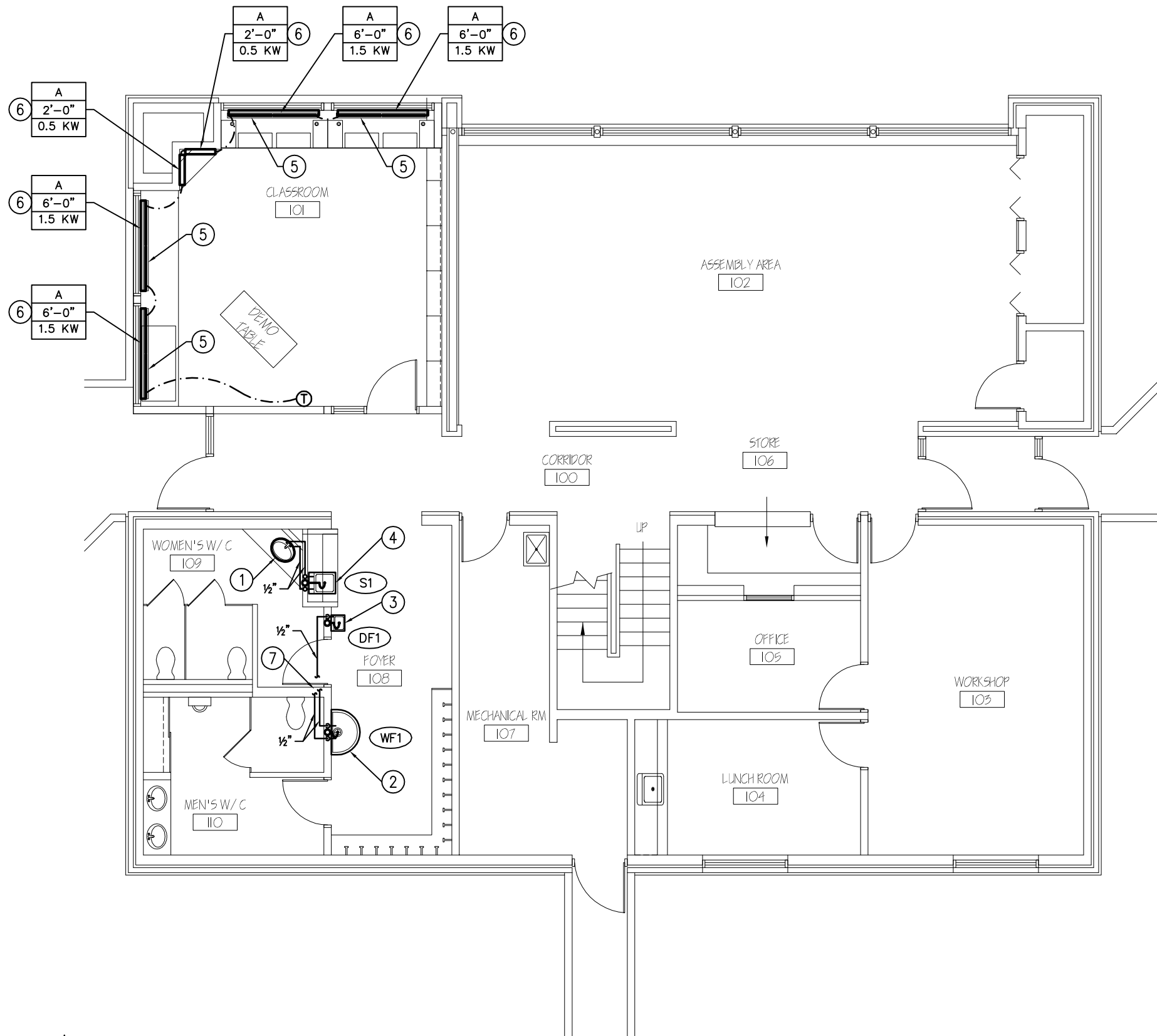
FLOOR PLAN - MECHANICAL SCALE: 1/8" = 1'-0"
