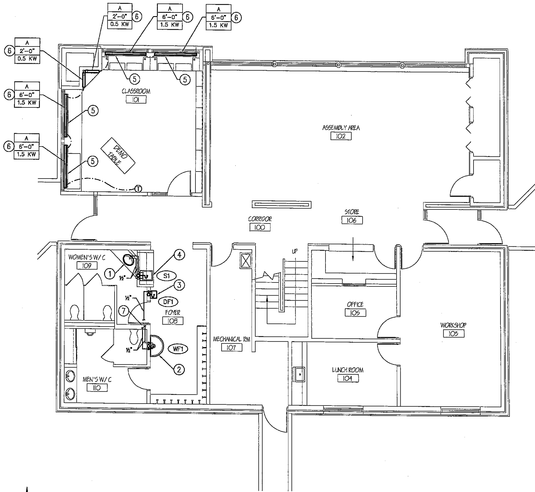
FLOOR PLAN - MECHANICAL SCALE: 1/8" = 1'-0"
