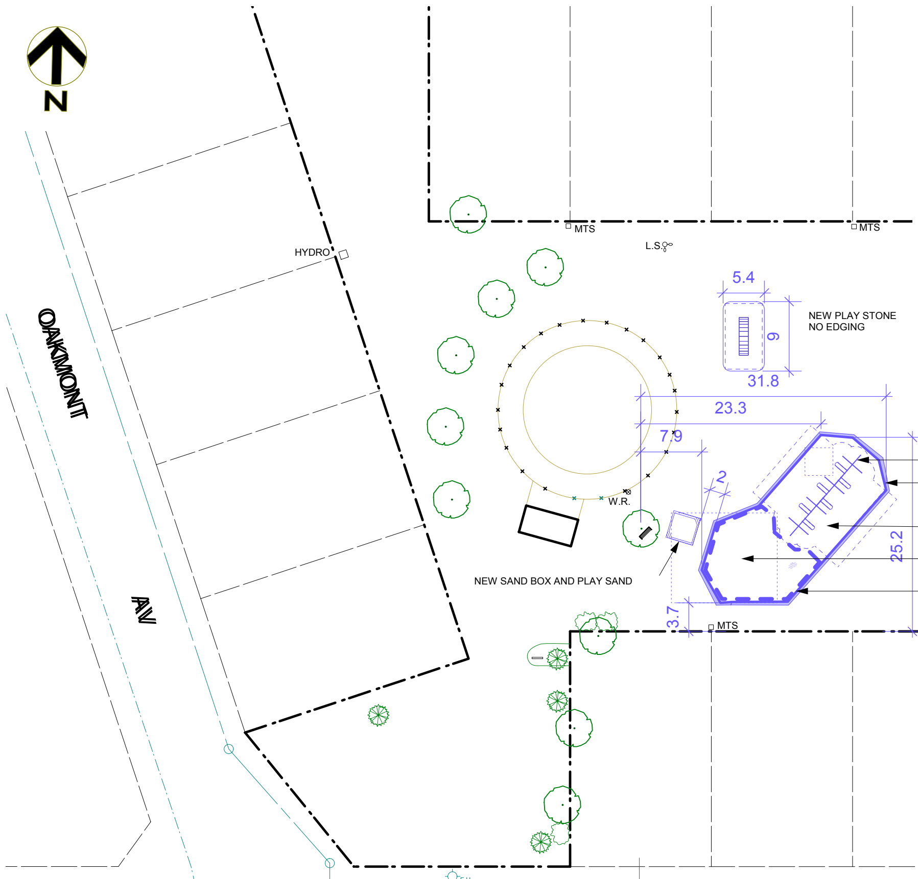
SAMPLE LAYOUT 1:400
