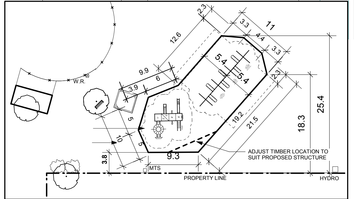
SAMPLE LAYOUT 1:400
