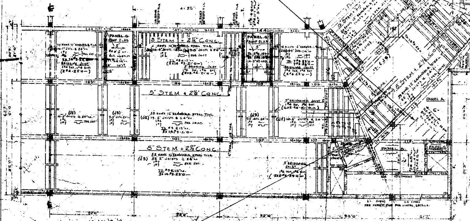
PART GROUND FLOOR PLAN 1/4" SCALE (PANELS A, B, C, & D)
