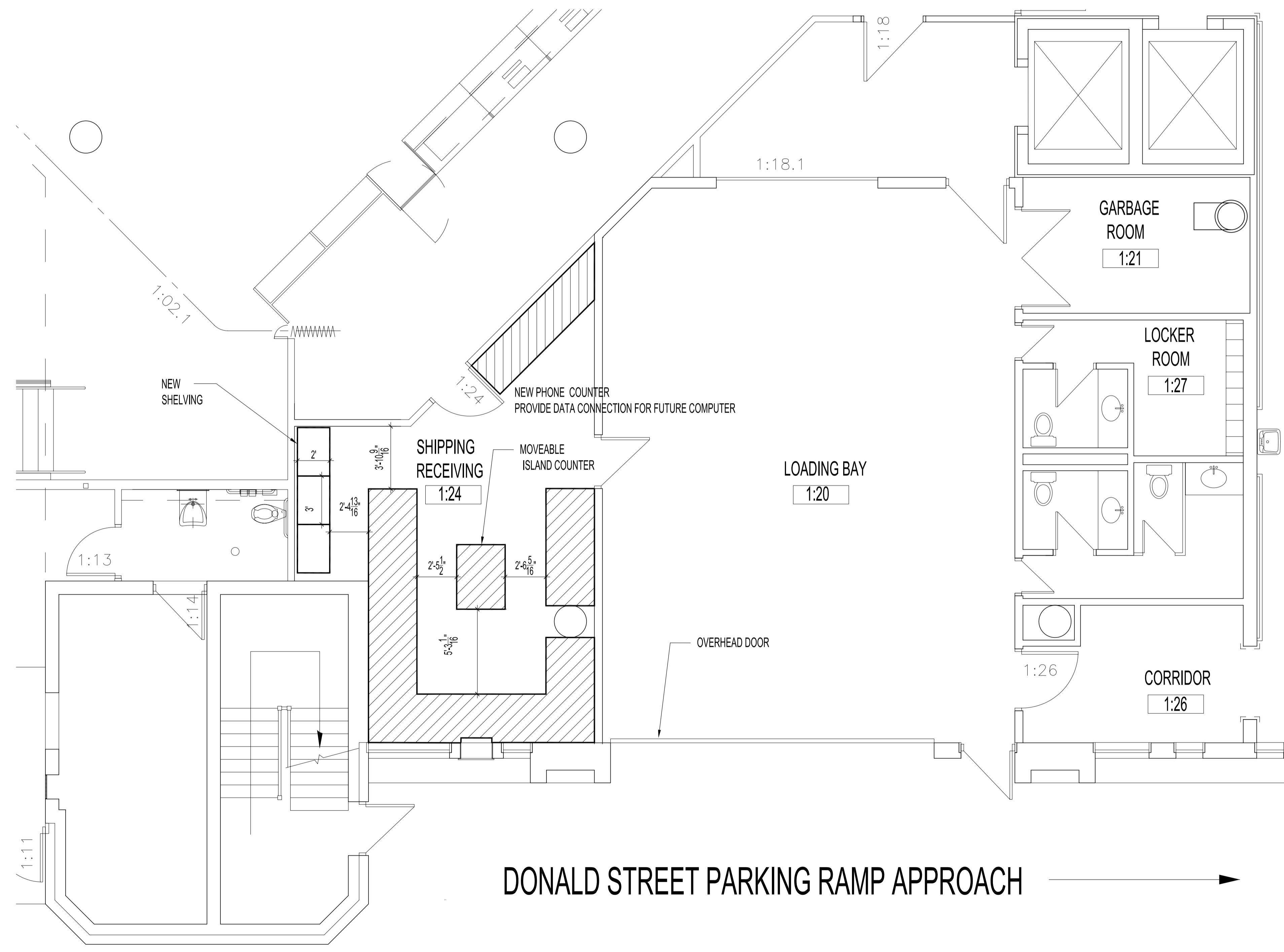
MAIN FLOOR PLAN - SHIPPING / RECEIVING SCALE: 1/4"=1'-0"
