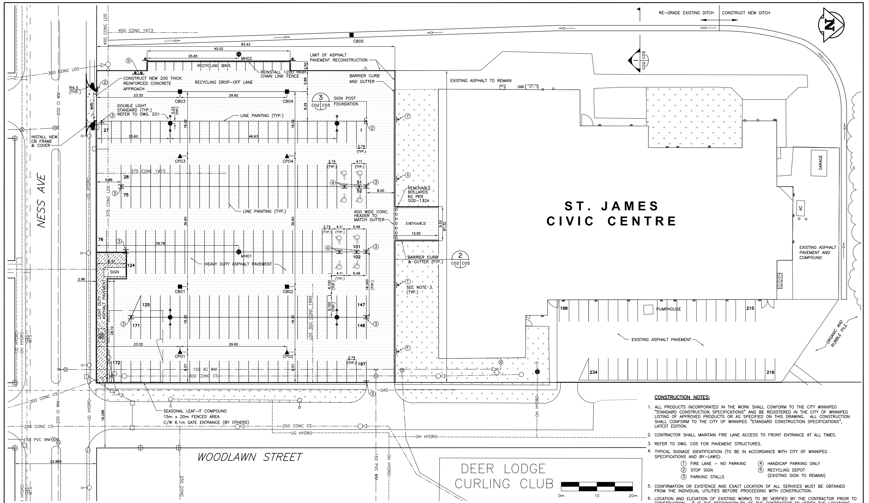
PROPOSED SITE PLAN SCALE 1:300
