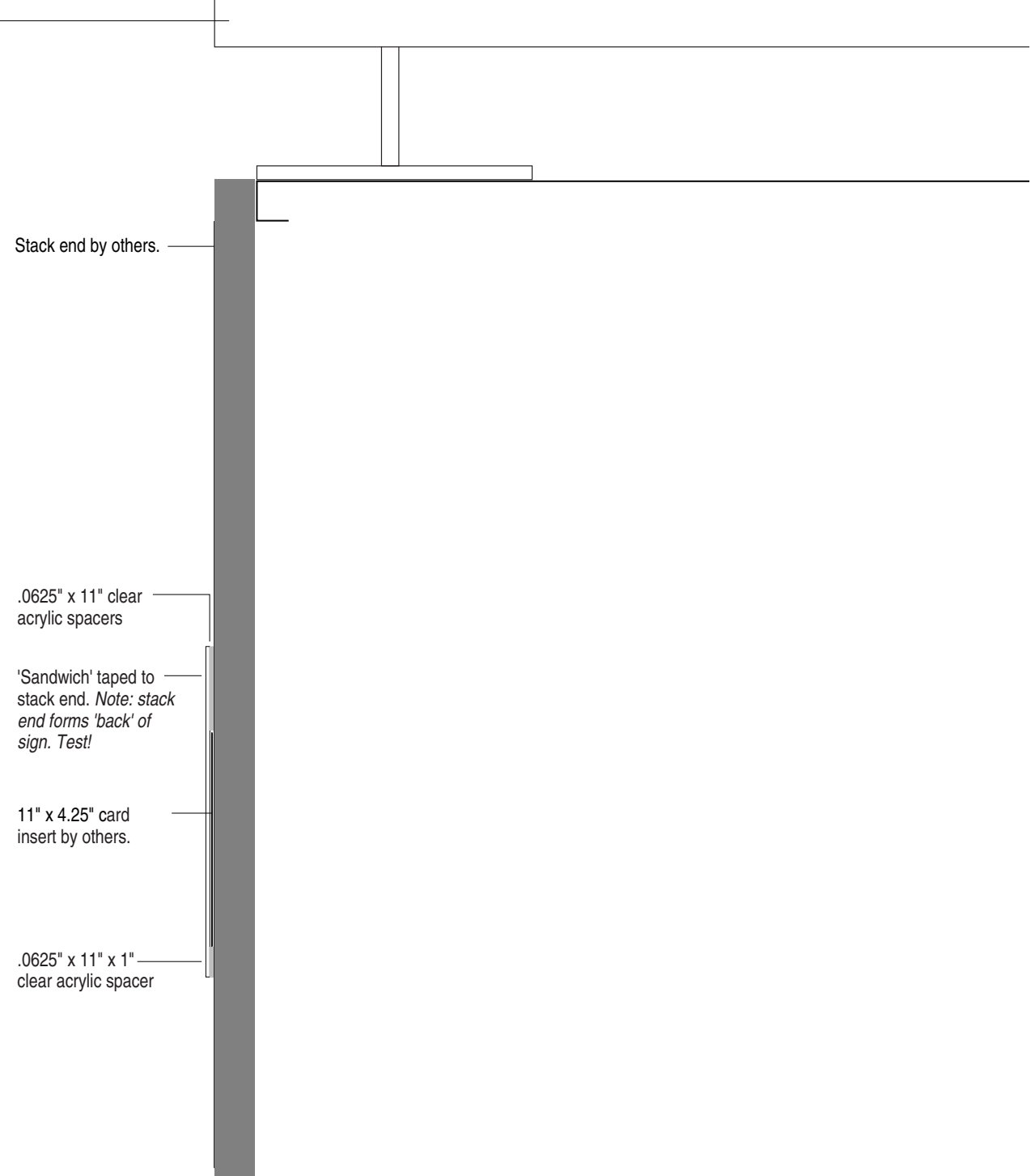
Section through Stack End Holder
