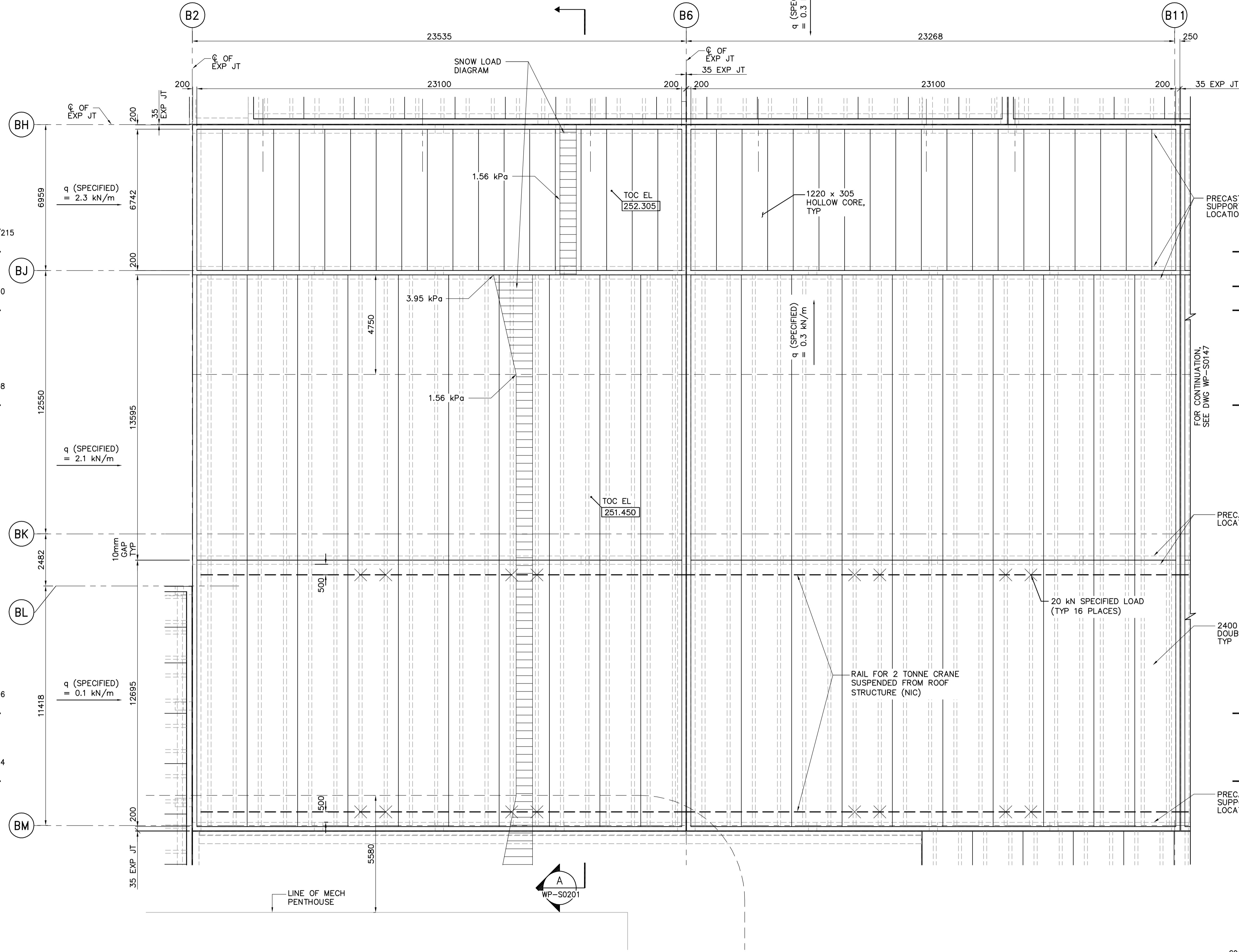
ROOF PLAN 1:100
