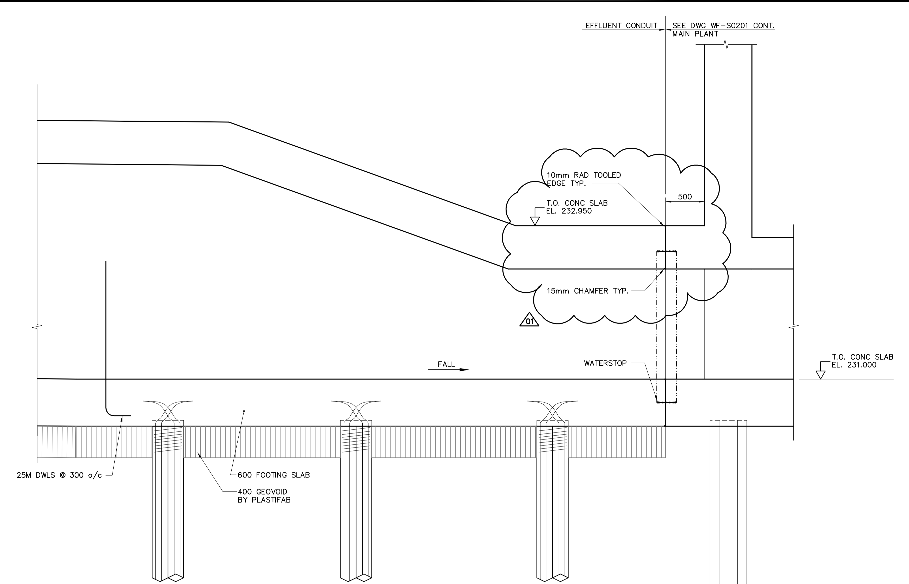
1 SECTION WT-S041 1:25
