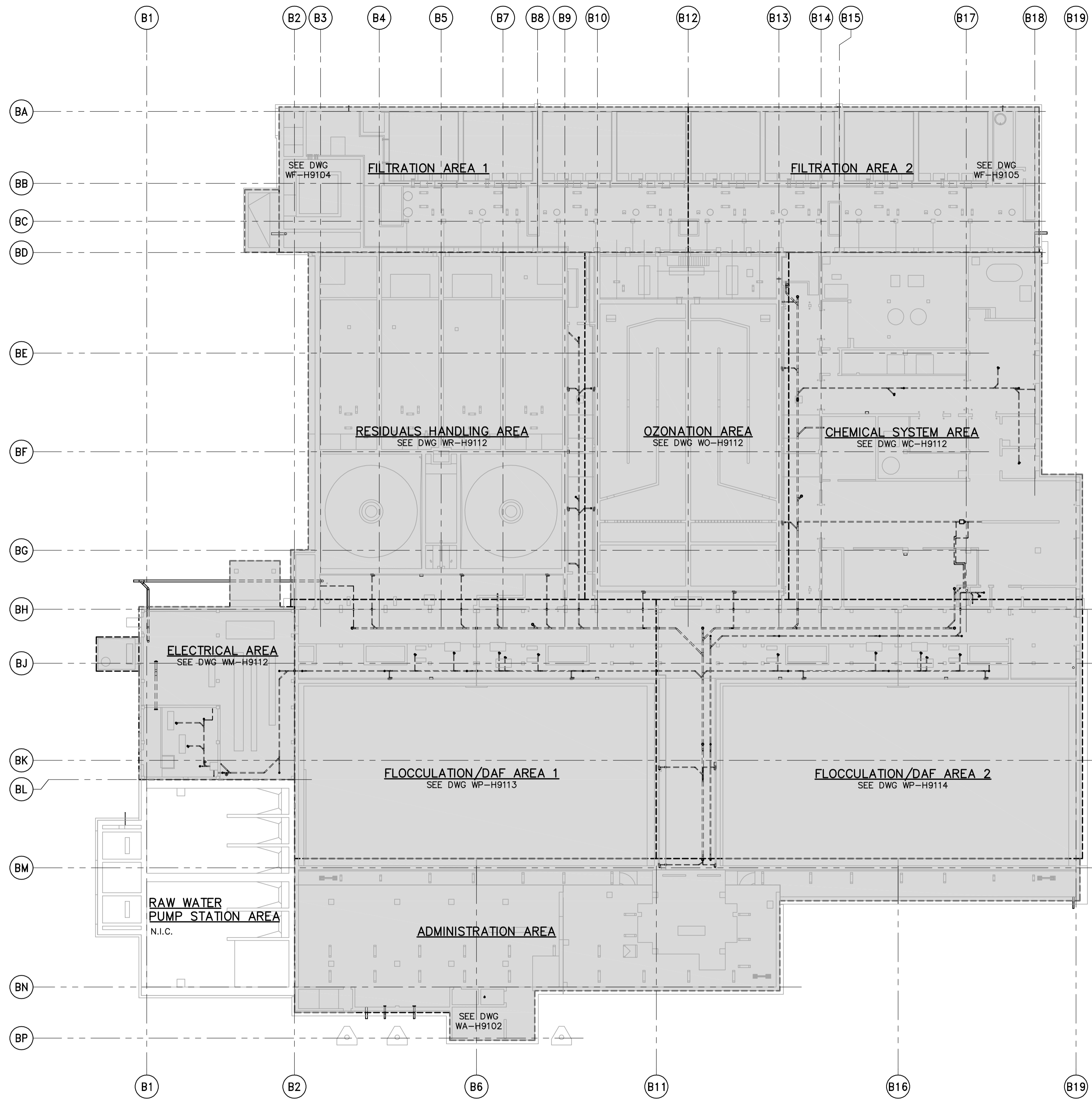
FIRST FLOOR PLAN 1:300
