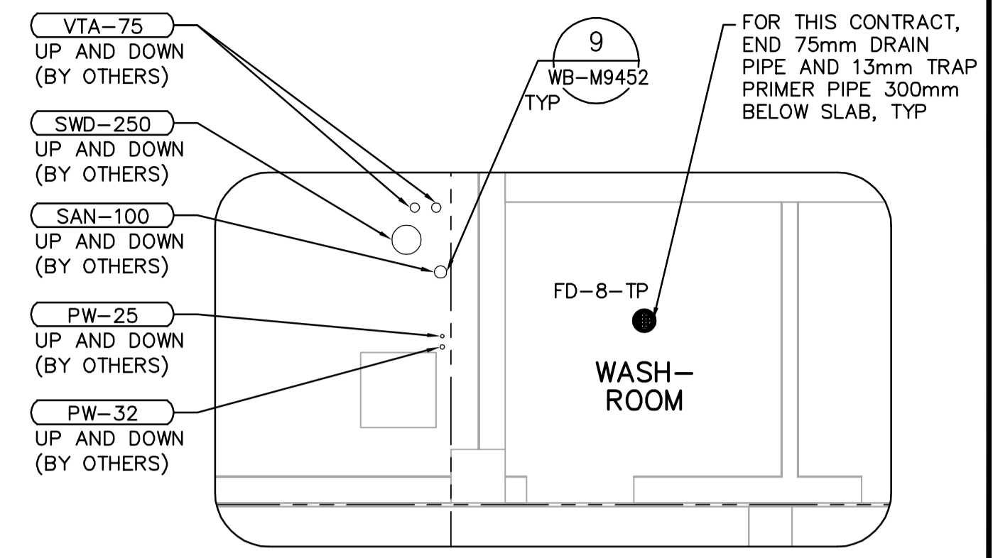
1 - 1:50 DETAIL
