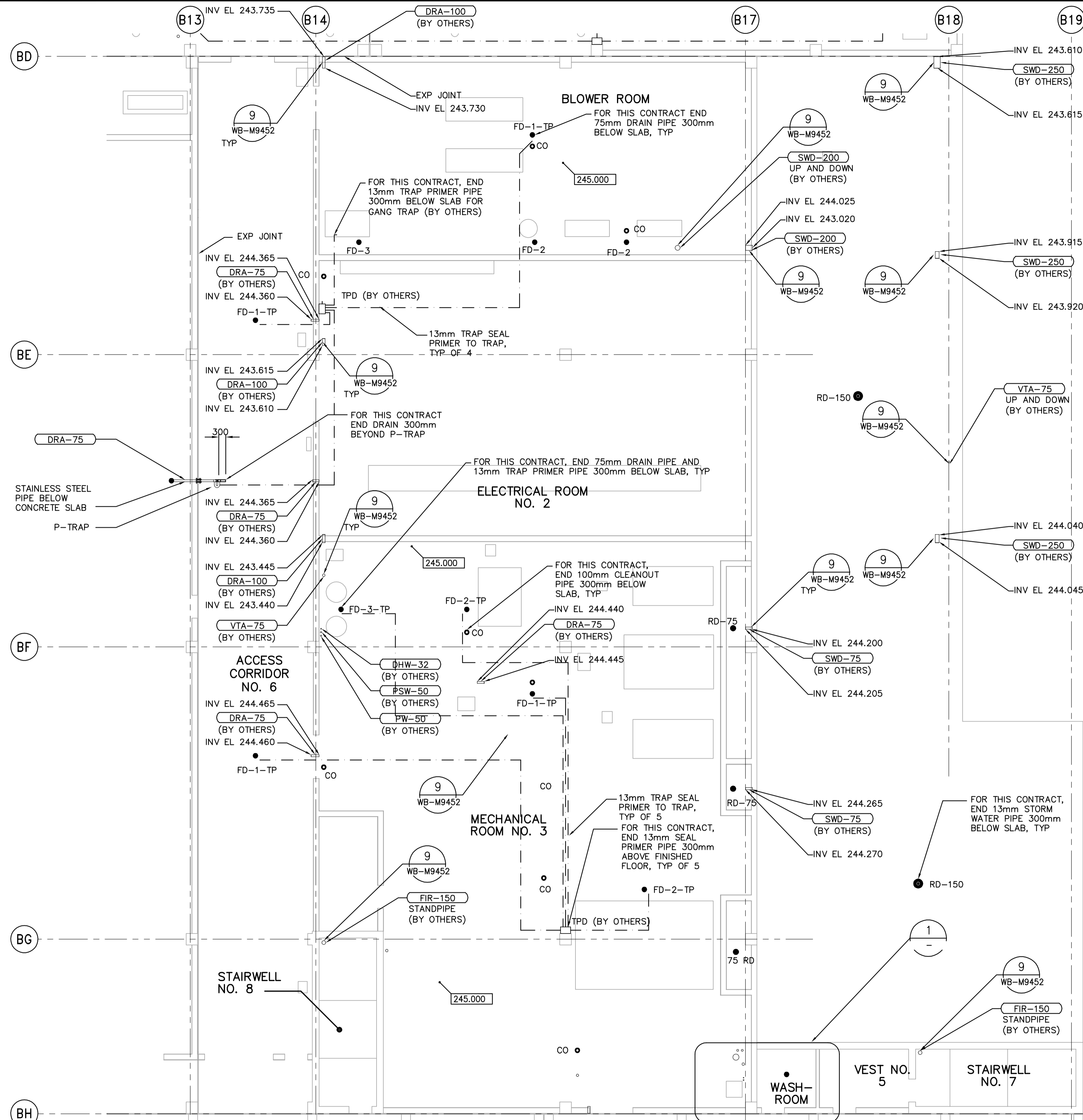
THIRD FLOOR PLAN 1:100
