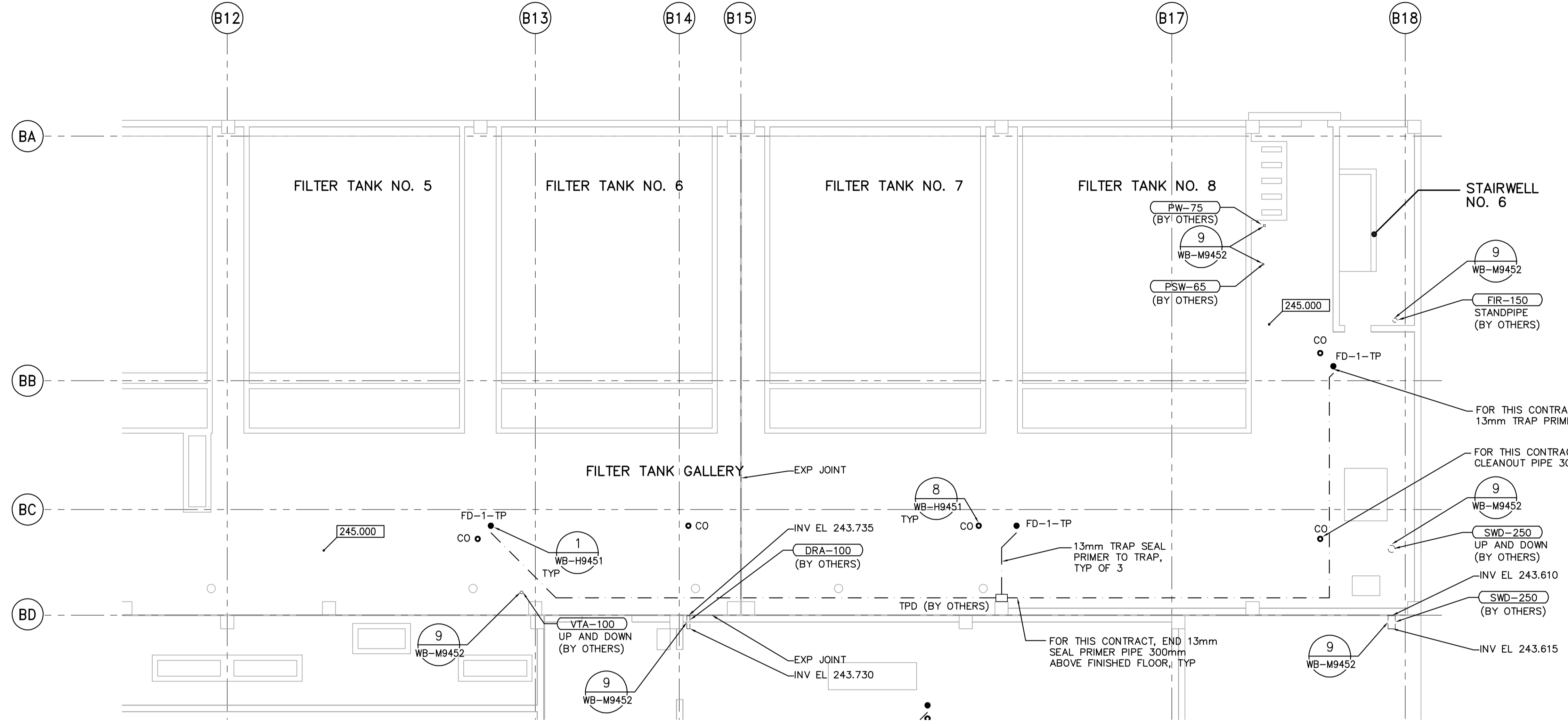
THIRD FLOOR PLAN 1:100
