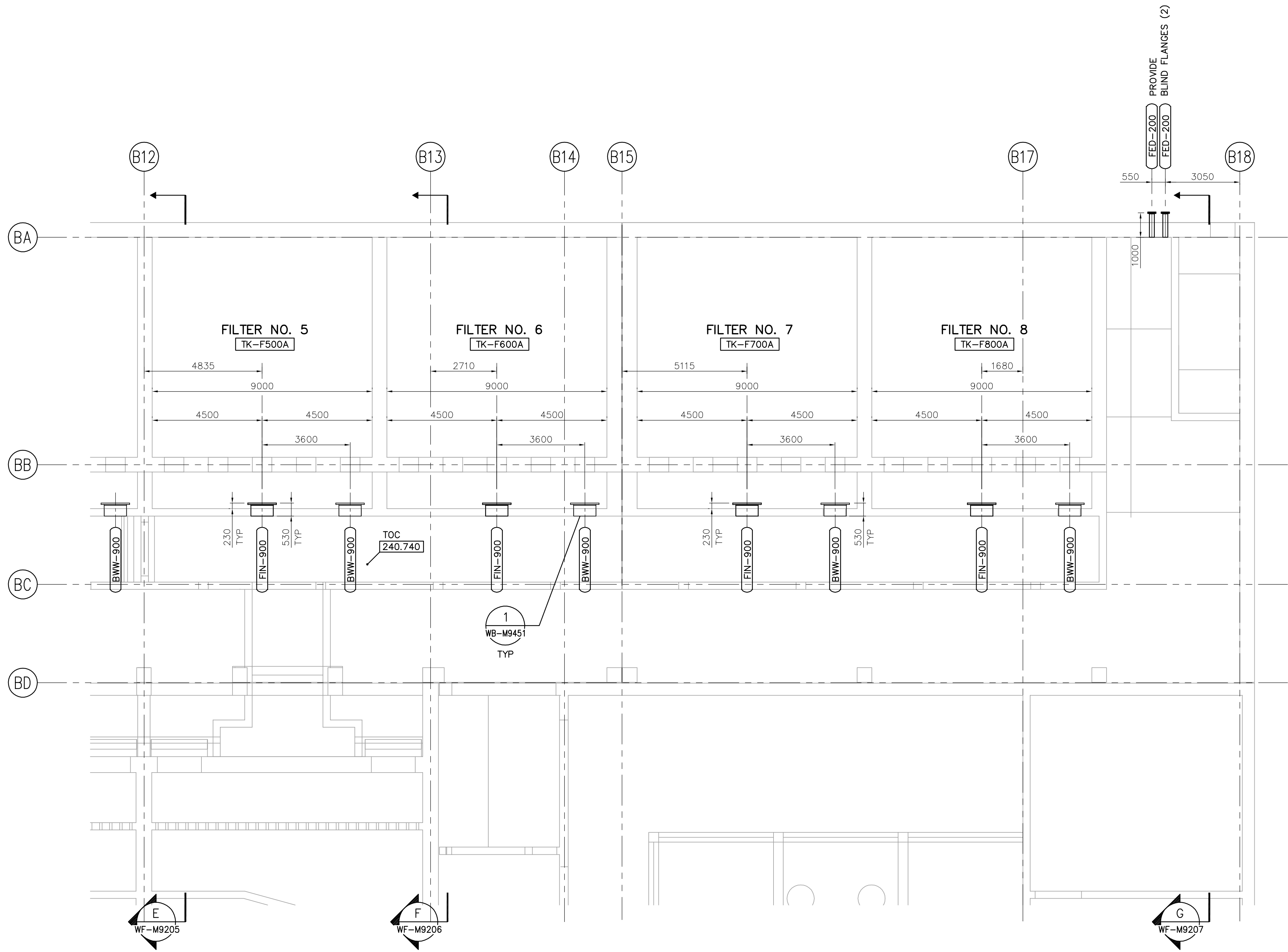
PLAN AT ELEVATION 240.740 1:100
