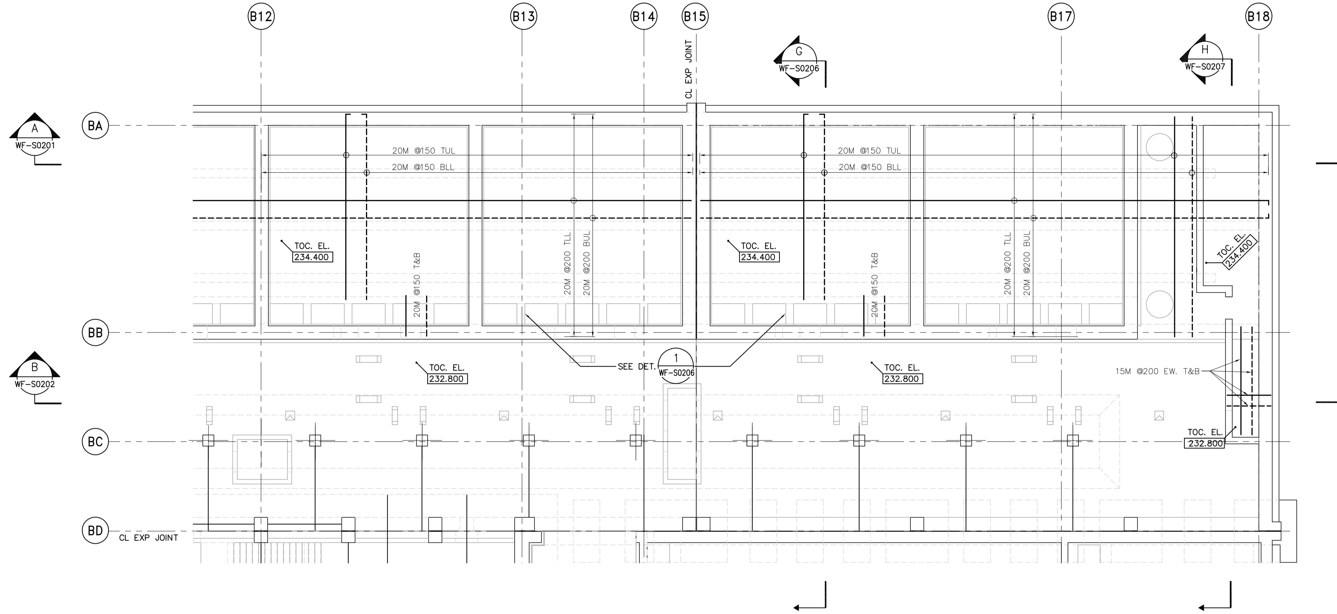
PLAN AT EL. 234.400 1:100
