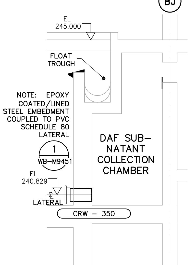
B SECTION - DAF LATERALS - TYP. 64 WP-M9101 1:50
