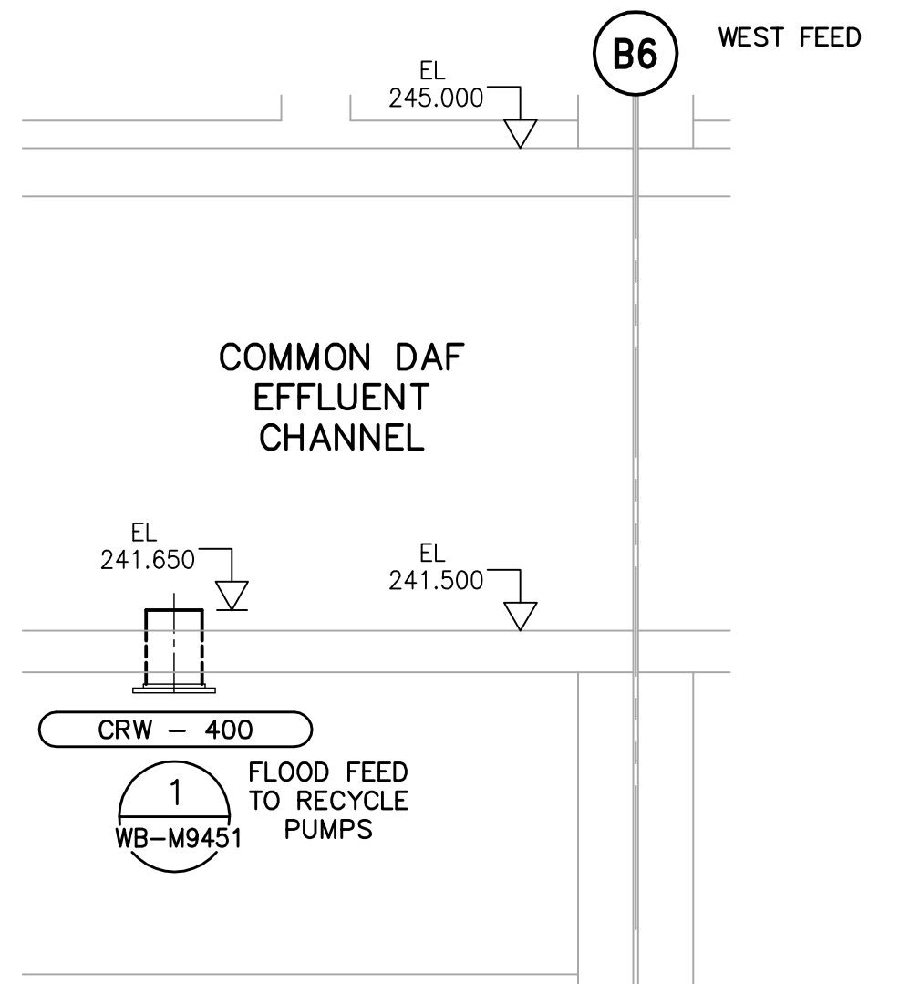
D SECTION - FEEDS TO RECYCLE PUMPS - TYP. 2 WP-M9101 1:50
