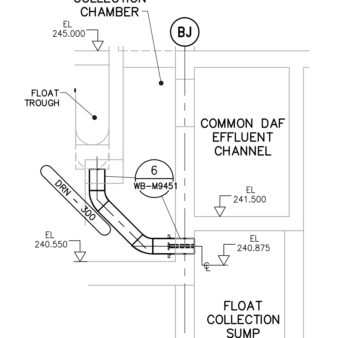
C SECTION - FLOAT TROUGH DRAINS TO FLOAT SUMPS TYP. 8 WP-M9101 1:50
