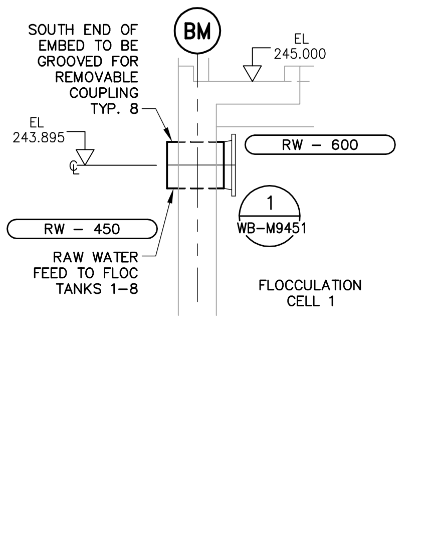
A SECTION - RAW WATER FEEDS TO FLOC TANKS - TYP. 8 WP-M9101 1:50
