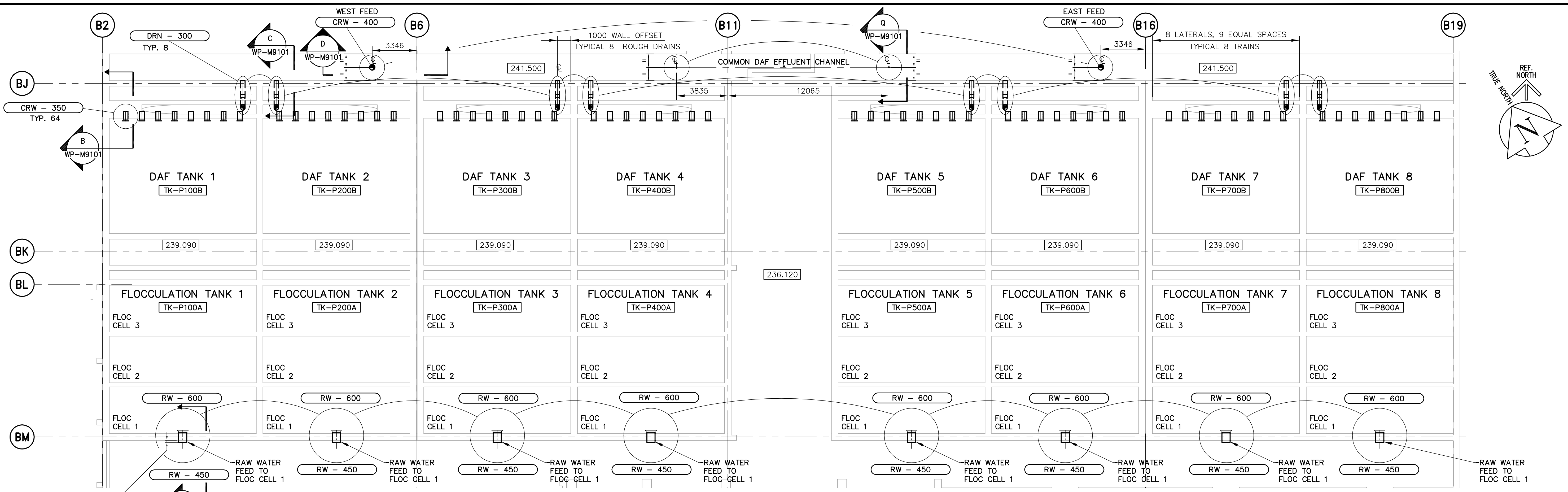
15 PLAN AT EL. 244.400 WP-M9101 1:150
